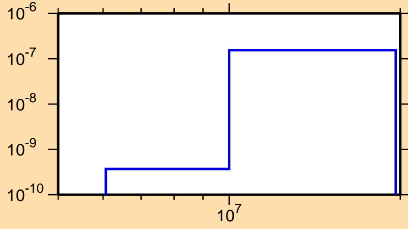
\sigma vs. E for ^{215}\text{Th}(\text{mt } 45)
