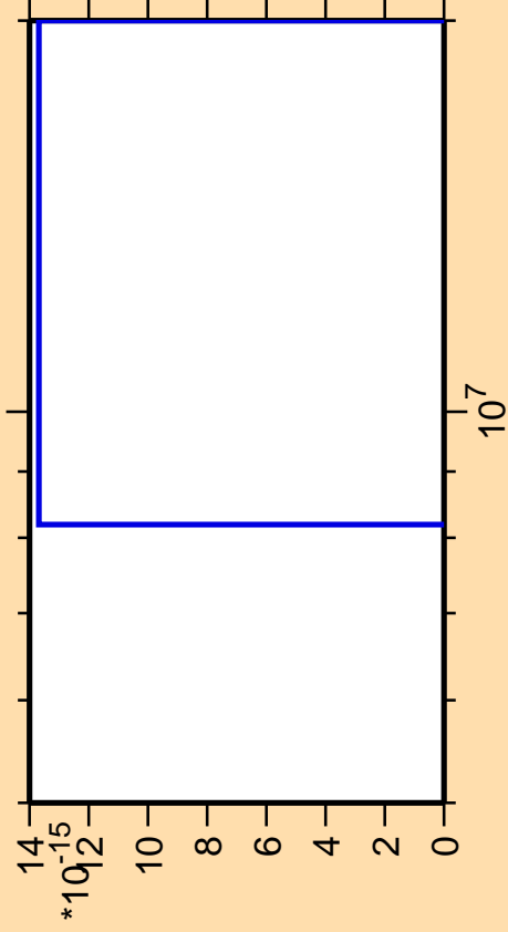
\Delta\sigma/\sigma vs. E for ^{215}\text{Th} (mt 42)
