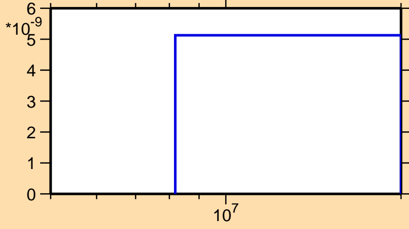
\sigma vs. E for ^{215}\text{Th}(\text{mt117})
