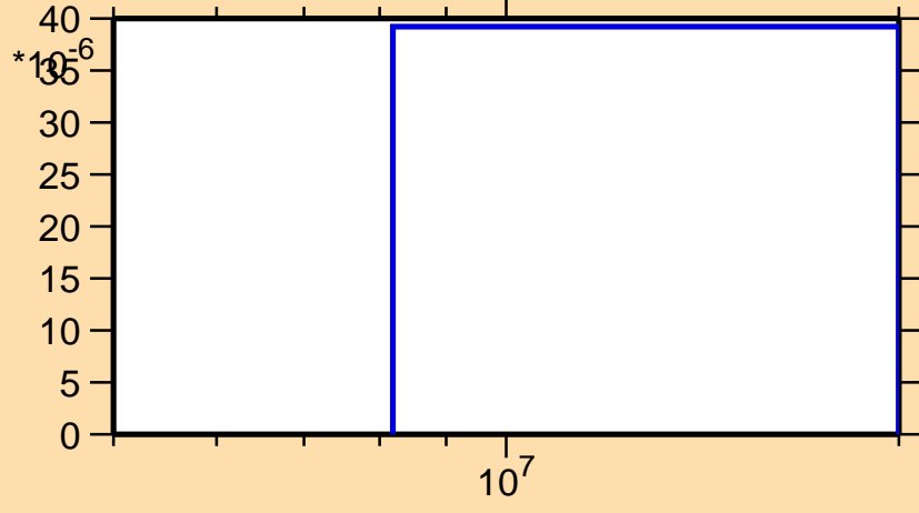
\sigma vs. E for ^{215}\text{Th}(n,3n)
