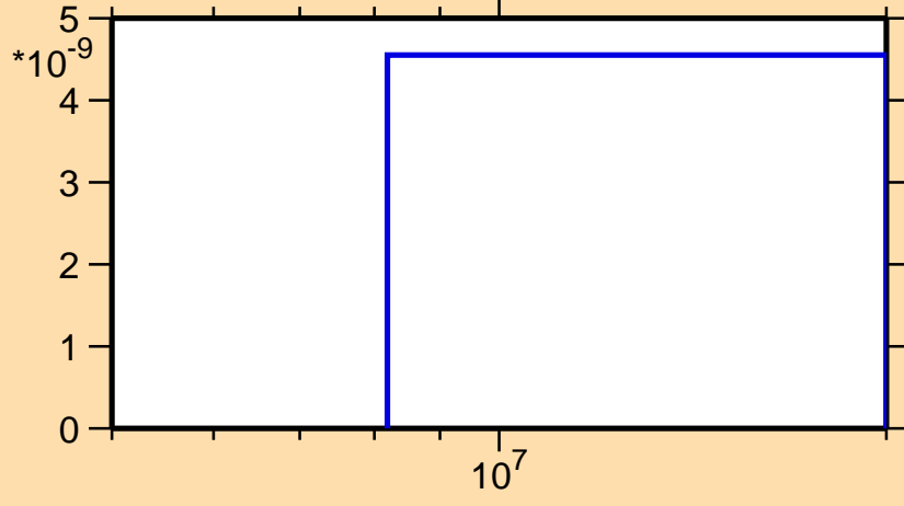
\sigma vs. E for ^{215}\text{Th}(n,pd)
