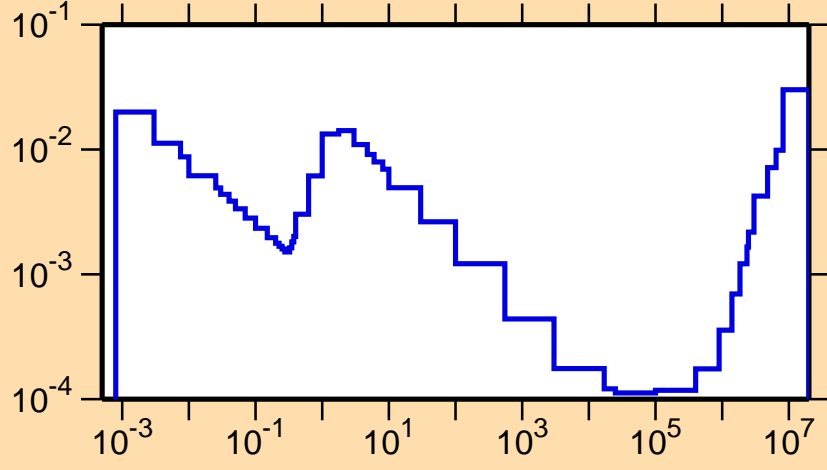
\sigma vs. E for ^{215}\text{Th}(n,p)
