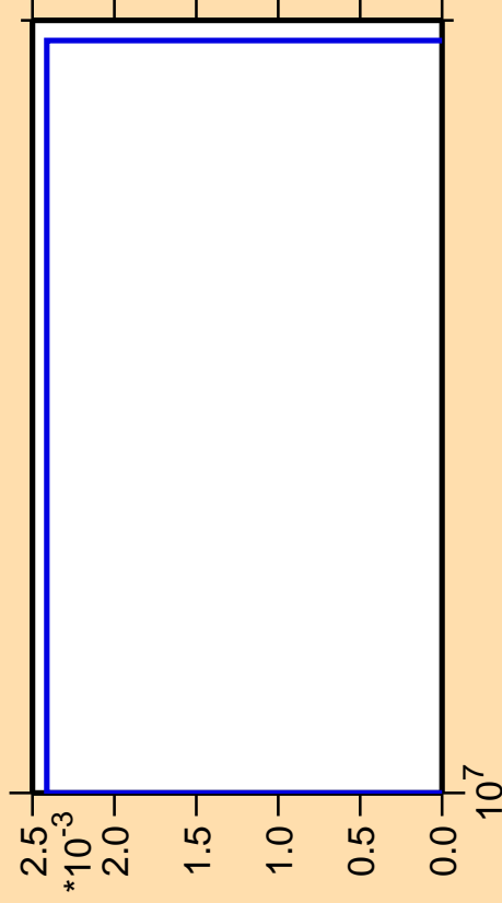
\Delta\sigma/\sigma vs. E for ^{225}\text{Th} (mt 11)
