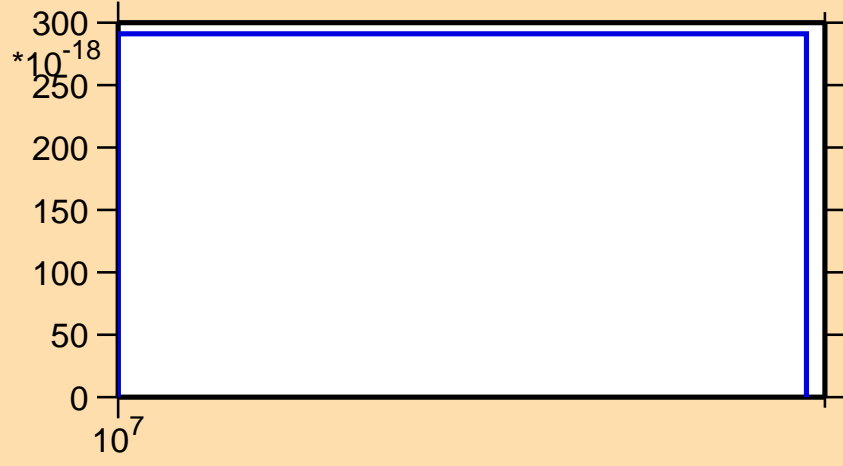
\sigma vs. E for ^{225}\text{Th} (mt 11)
