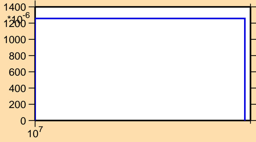
\sigma vs. E for ^{225}\text{Th}(n,3n\alpha)
