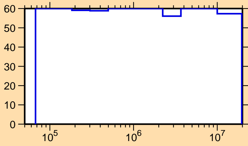
\Delta\sigma/\sigma vs. E for ^{225}\text{Th}(n,n_1)
