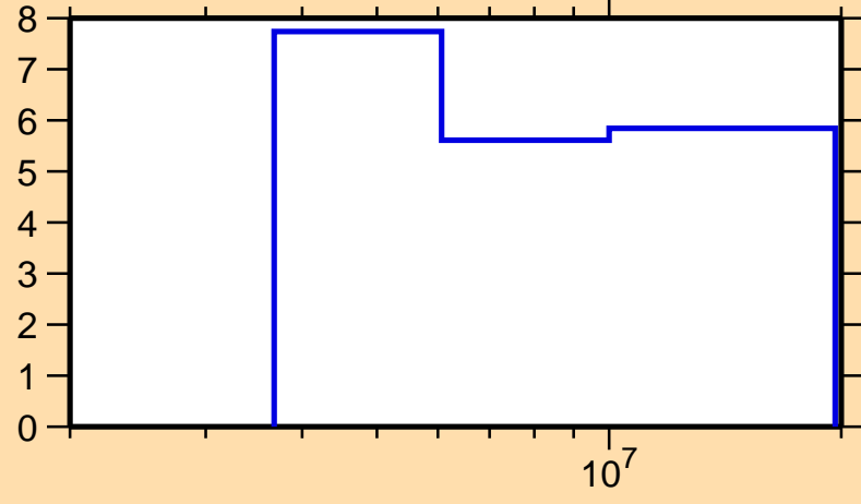
\Delta\sigma/\sigma vs. E for ^{225}\text{Th}(n,\text{nonel.})
