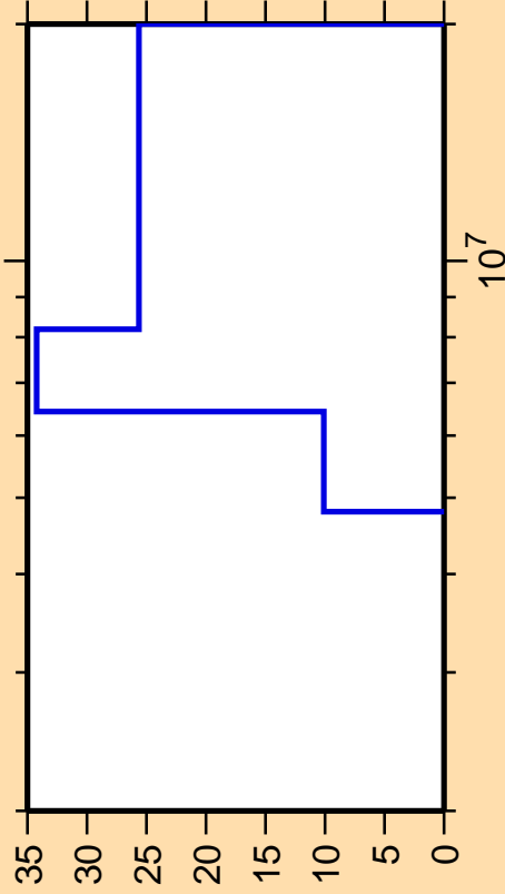
\Delta\sigma/\sigma vs. E for ^{225}\text{Th}(n,n\text{cont.})
