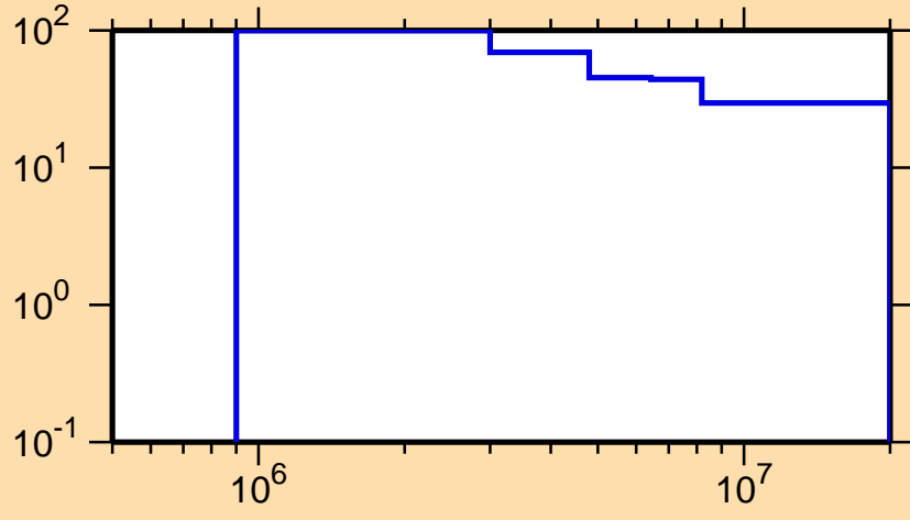
\Delta\sigma/\sigma vs. E for ^{225}\text{Th}(n,p)
