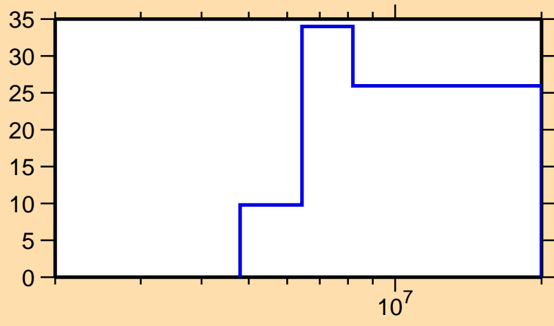
\Delta\sigma/\sigma vs. E for ^{225}\text{Th}(n,\text{inel.})
