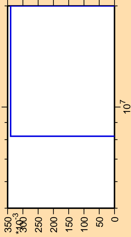
\Delta\sigma/\sigma vs. E for ^{225}\text{Th}(\text{mt117})
