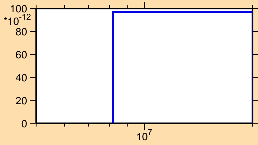
\sigma vs. E for ^{225}\text{Th}(n,p\alpha)
