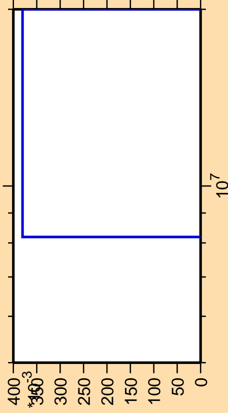
\Delta\sigma/\sigma vs. E for ^{225}\text{Th} (mt 45)
