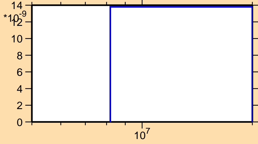
\sigma vs. E for ^{225}\text{Th}(n,nt)
