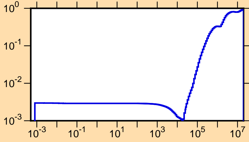
\mu vs. E for ^{226}\text{Th}(\text{mt251})
