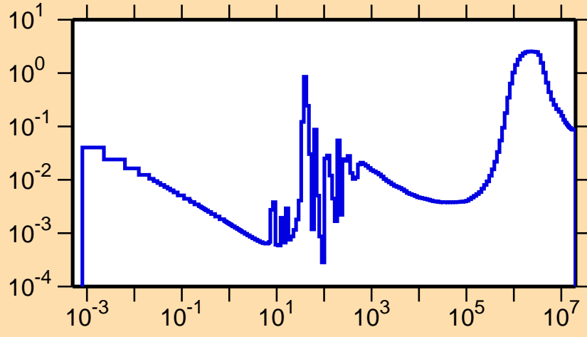
\sigma vs. E for ^{226}\text{Th}(n,f)
