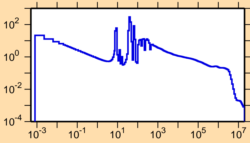
\sigma vs. E for ^{226}\text{Th}(n,\gamma)
