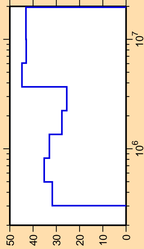
\Delta\sigma/\sigma vs. E for ^{226}\text{Th}(n,n_4)
