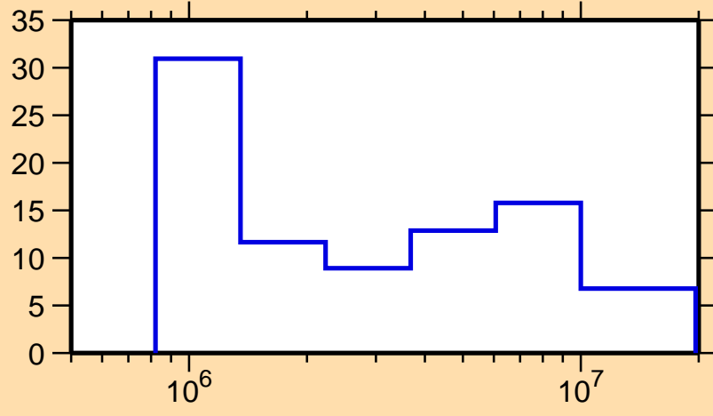
\Delta\sigma/\sigma vs. E for ^{226}\text{Th}(n,\text{el.})
