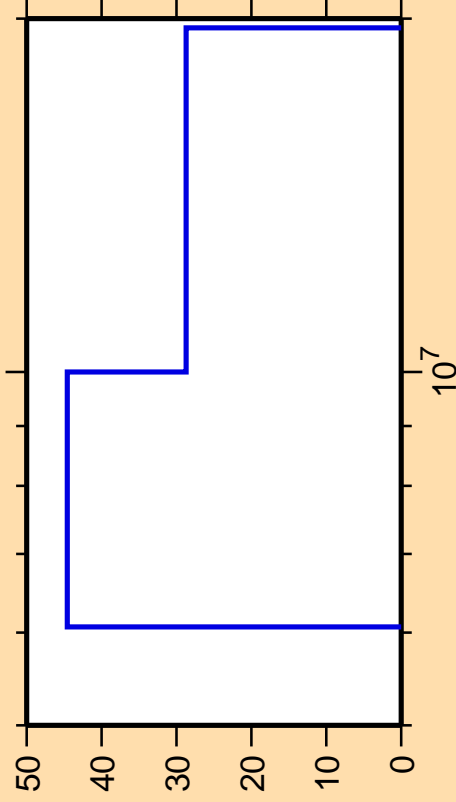
\Delta\sigma/\sigma vs. E for ^{226}\text{Th}(n,d)
