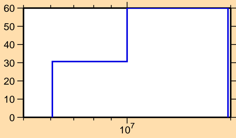
\Delta\sigma/\sigma vs. E for ^{226}\text{Th}(n,\text{inel.})
