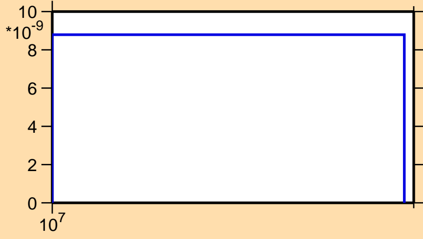
\sigma vs. E for ^{226}\text{Th}(n,nt)
