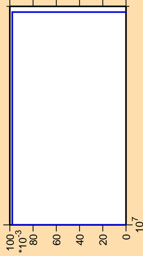
\Delta\sigma/\sigma vs. E for ^{226}\text{Th} (mt 45)
