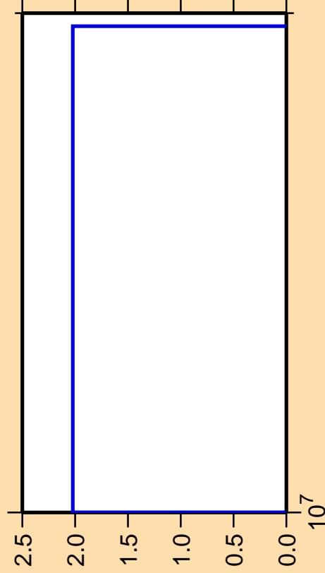
\Delta\sigma/\sigma vs. E for ^{226}\text{Th}(n,p\alpha)
