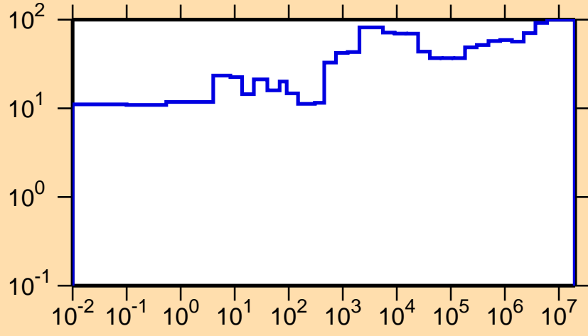
\Delta\sigma/\sigma vs. E for ^{226}\text{Th}(n,\gamma)
