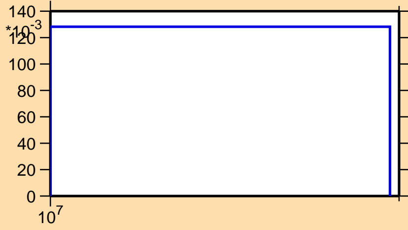
\sigma vs. E for ^{226}\text{Th}(n,3n)
