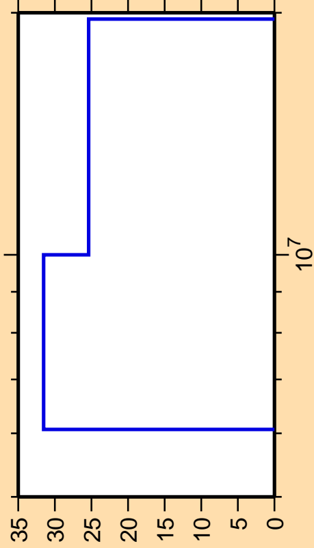
\Delta\sigma/\sigma vs. E for ^{226}\text{Th}(n,2n)
