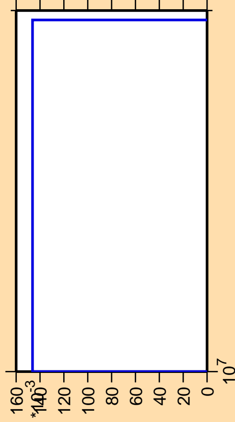
\Delta\sigma/\sigma vs. E for ^{226}\text{Th}(\text{mt117})
