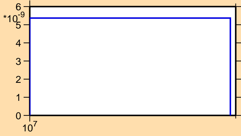
\sigma vs. E for ^{226}\text{Th}(n,2np)
