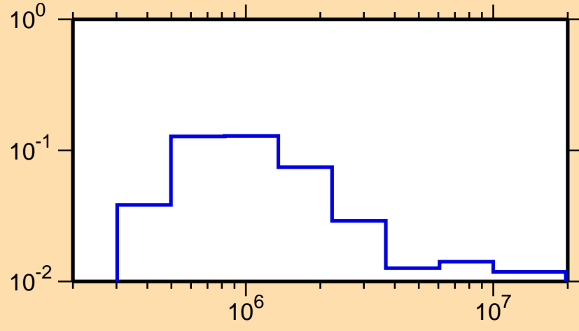
\sigma vs. E for ^{226}\text{Th}(n,n_4)
