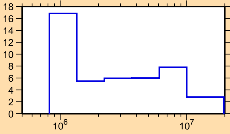
\Delta\sigma/\sigma vs. E for ^{226}\text{Th}(n,\text{tot.})
