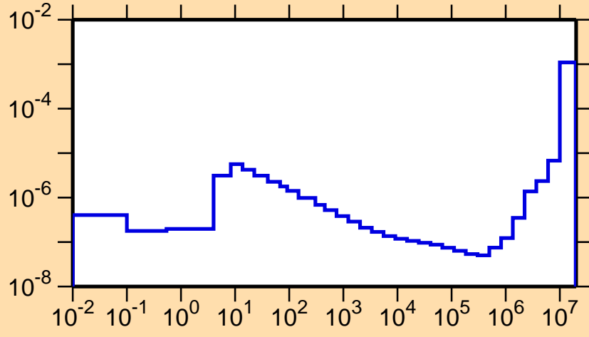
\sigma vs. E for ^{226}\text{Th}(n,\alpha)
