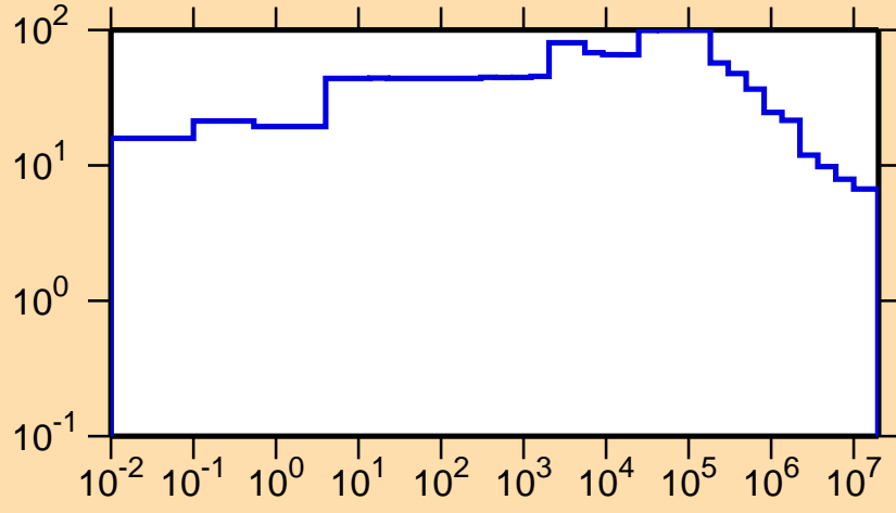
\Delta\sigma/\sigma vs. E for ^{226}\text{Th}(n,\text{nonel.})
