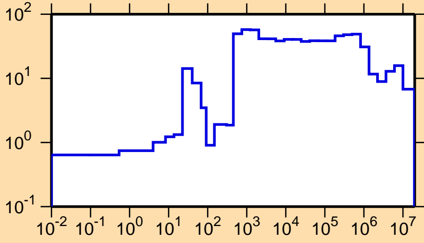
\Delta\sigma/\sigma vs. E for ^{226}\text{Th}(n,\text{el.})
