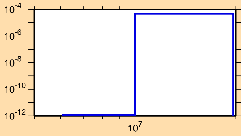
\sigma vs. E for ^{226}\text{Th}(n,t)
