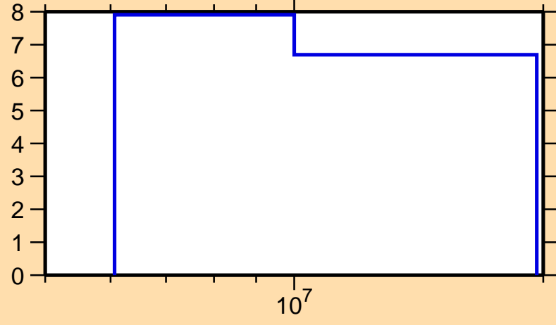
\Delta\sigma/\sigma vs. E for ^{226}\text{Th}(n,\text{nonel.})
