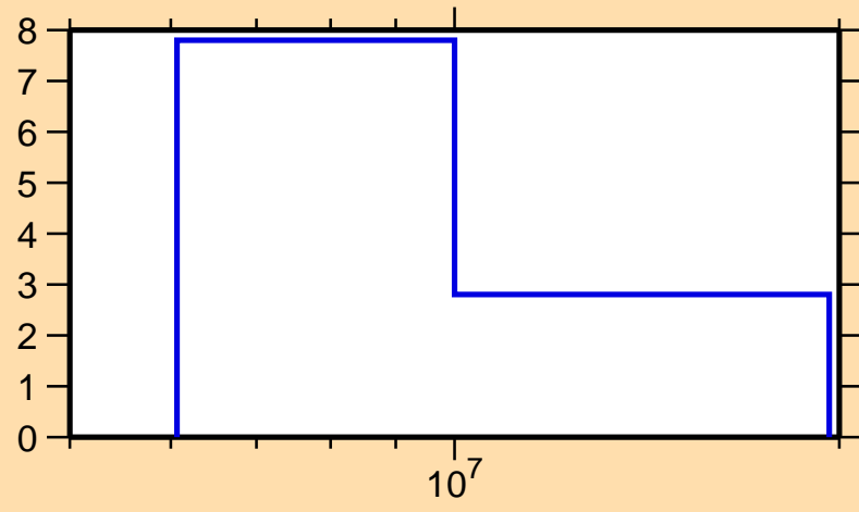
\Delta\sigma/\sigma vs. E for ^{226}\text{Th}(n,\text{tot.})
