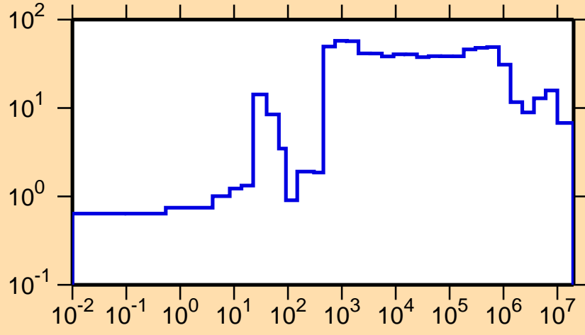
\Delta\sigma/\sigma vs. E for ^{226}\text{Th}(n,el.)
