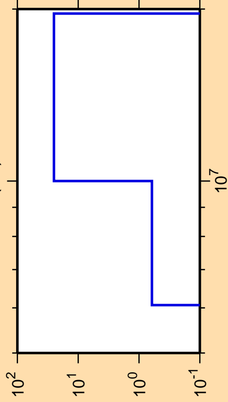
\Delta\sigma/\sigma vs. E for ^{226}\text{Th}(n,t)
