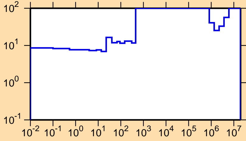
\Delta\sigma/\sigma vs. E for ^{226}\text{Th}(n,f)
