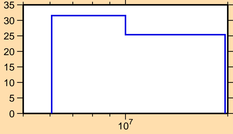
\Delta\sigma/\sigma vs. E for ^{226}\text{Th}(n,2n)
