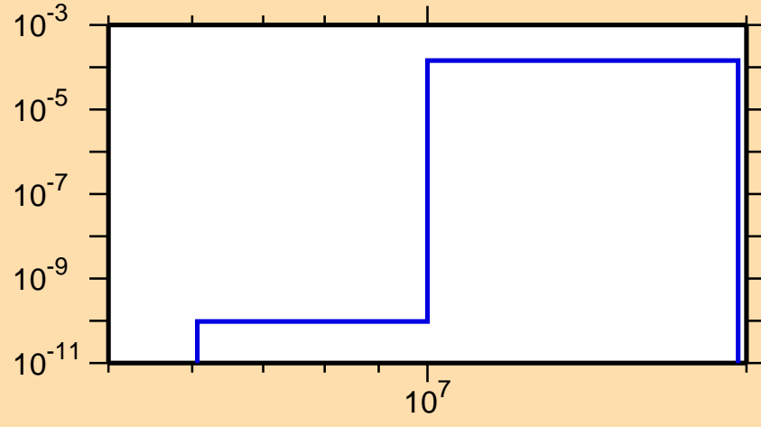
\sigma vs. E for ^{226}\text{Th}(n,d)
