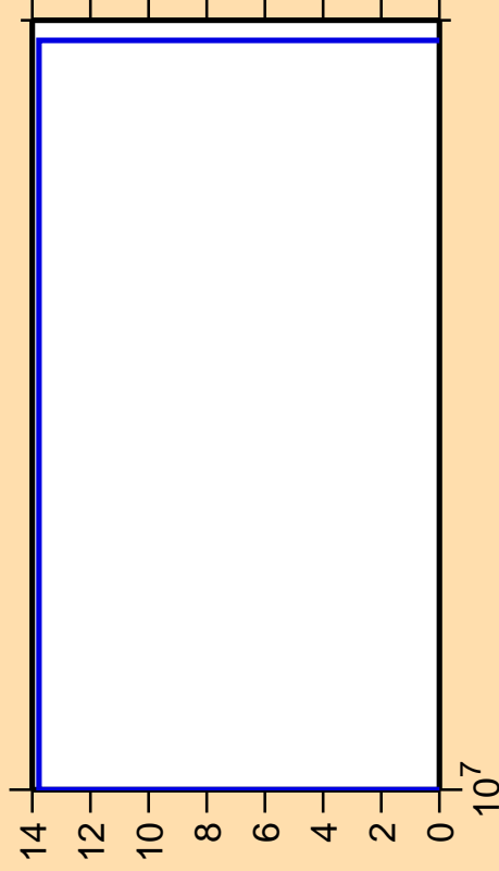
\Delta\sigma/\sigma vs. E for ^{226}\text{Th}(n,\text{He3})
