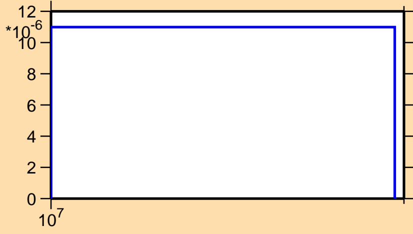
\sigma vs. E for ^{226}\text{Th}(n,3n\alpha)
