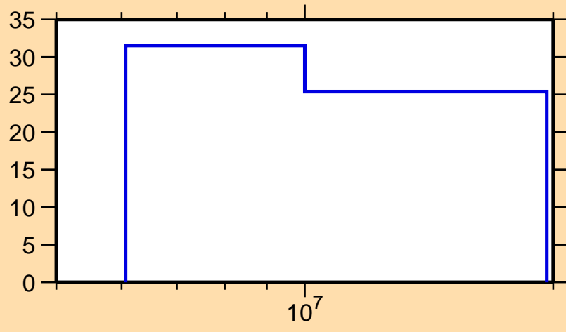
\Delta\sigma/\sigma vs. E for ^{226}\text{Th}(n,2n)
