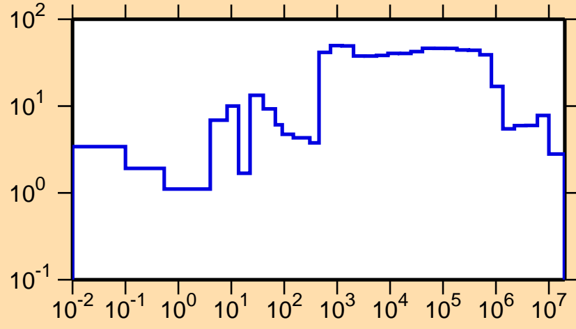
\Delta\sigma/\sigma vs. E for ^{226}\text{Th}(n,\text{tot.})
