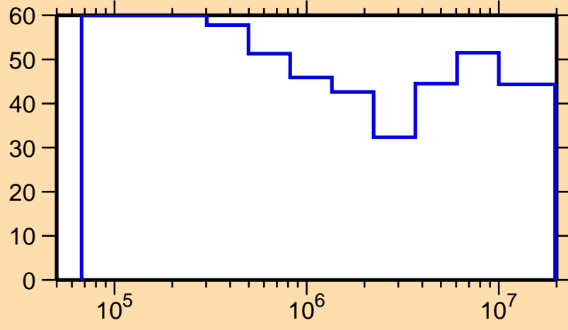
\Delta\sigma/\sigma vs. E for ^{226}\text{Th}(n,n_1)
