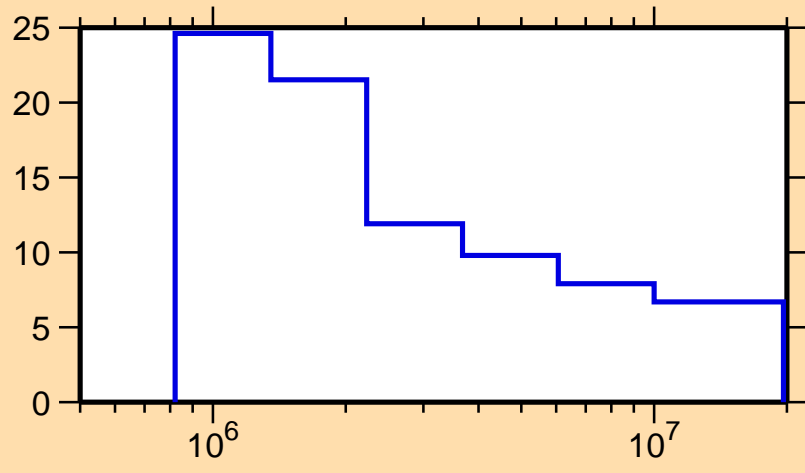
\Delta\sigma/\sigma vs. E for ^{226}\text{Th}(n,\text{nonel.})
