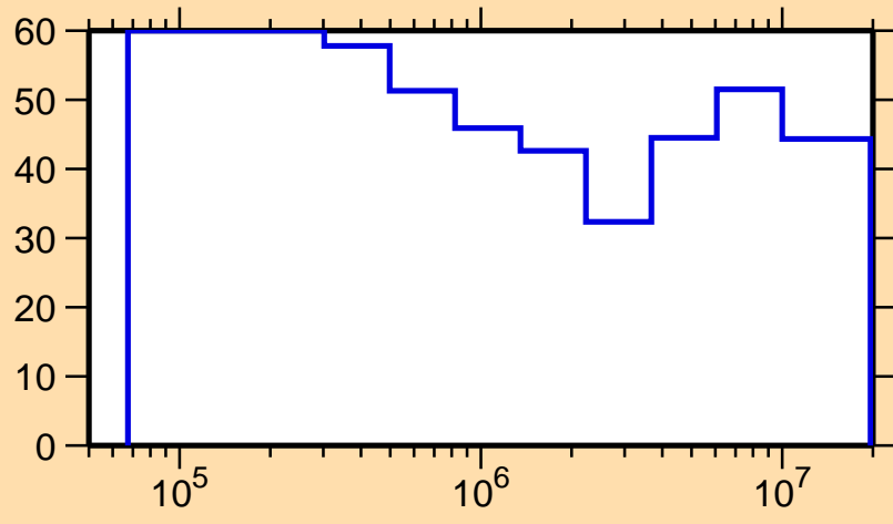
\Delta\sigma/\sigma vs. E for ^{226}\text{Th}(n,n_1)
