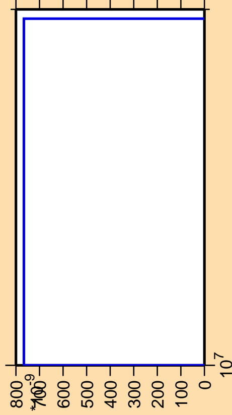
\Delta\sigma/\sigma vs. E for ^{226}\text{Th} (mt 42)
