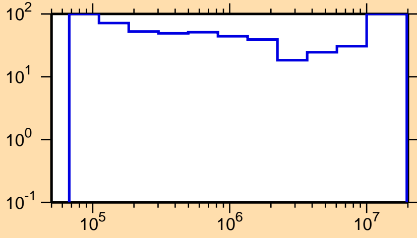
\Delta\sigma/\sigma vs. E for ^{226}\text{Th}(n,\text{inel.})
