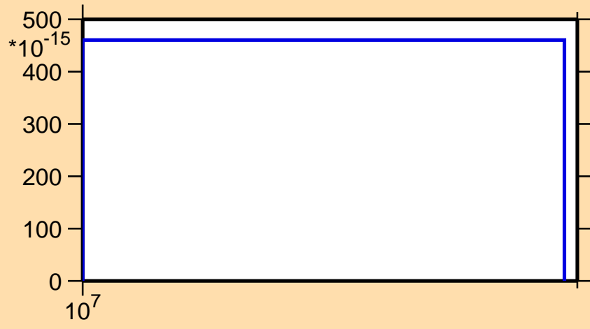
\sigma vs. E for ^{226}\text{Th}(n,p\alpha)
