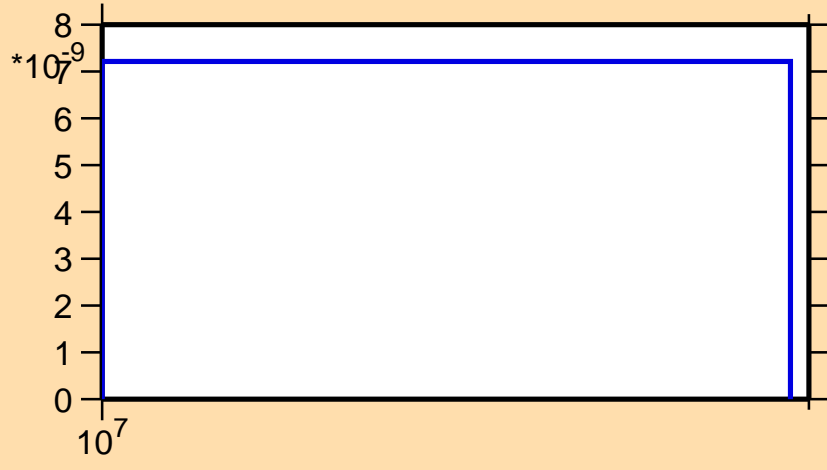
\sigma vs. E for ^{226}\text{Th}(n,\text{nd})
