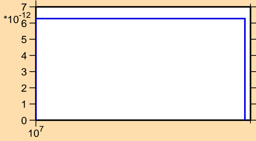
\sigma vs. E for ^{226}\text{Th}(n,\text{He3})
