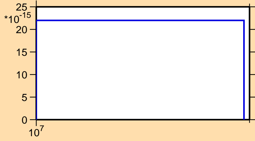
\sigma vs. E for ^{226}\text{Th}(\text{mt117})
