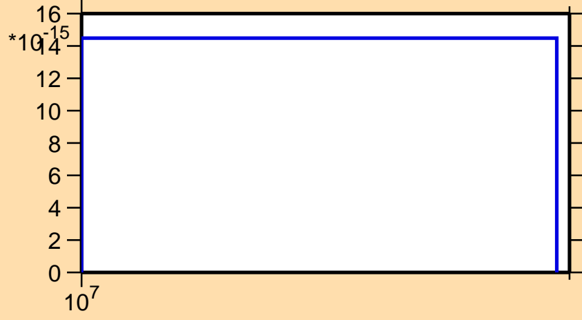
\sigma vs. E for ^{226}\text{Th} (mt 45)
