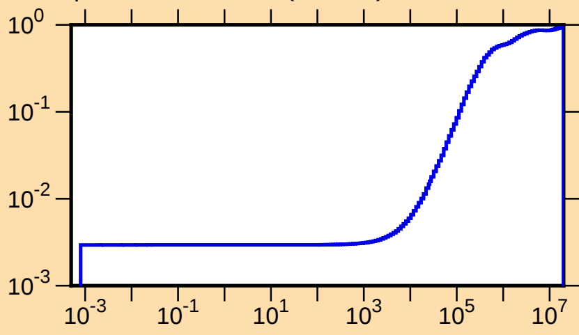
\mu vs. E for ^{229}\text{Th}(\text{mt251})
