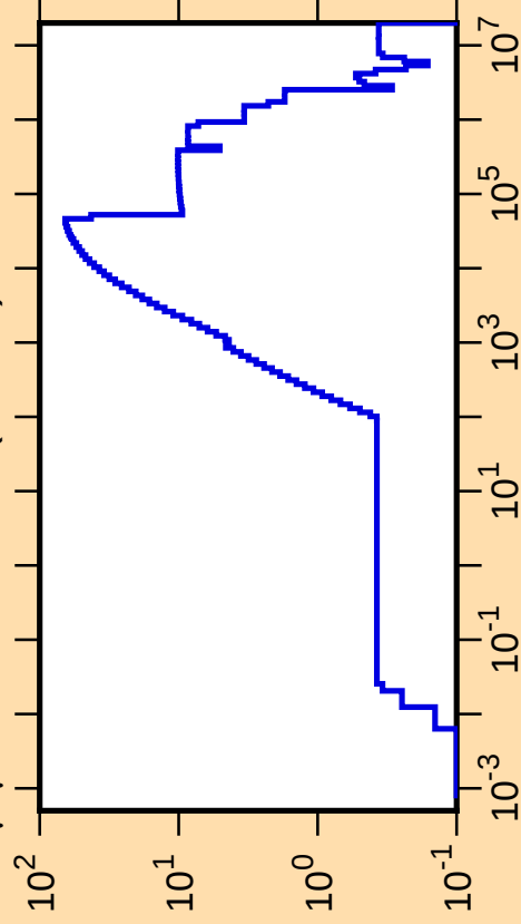
\Delta\mu/\mu vs. E for ^{229}\text{Th}(\text{mt251})
