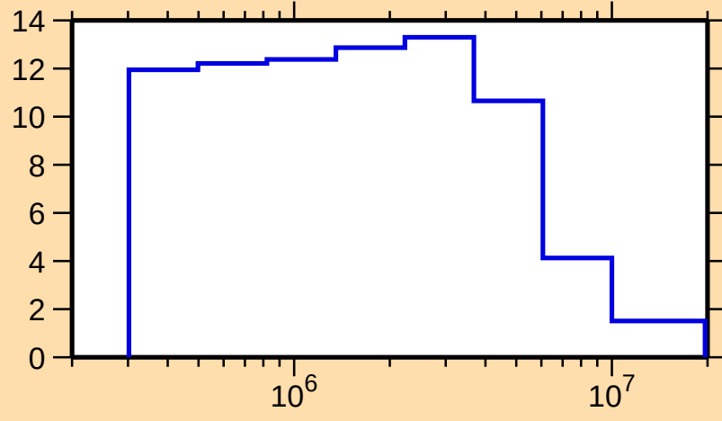
\Delta\sigma/\sigma vs. E for ^{229}\text{Th}(\text{n},\text{nonel.})
