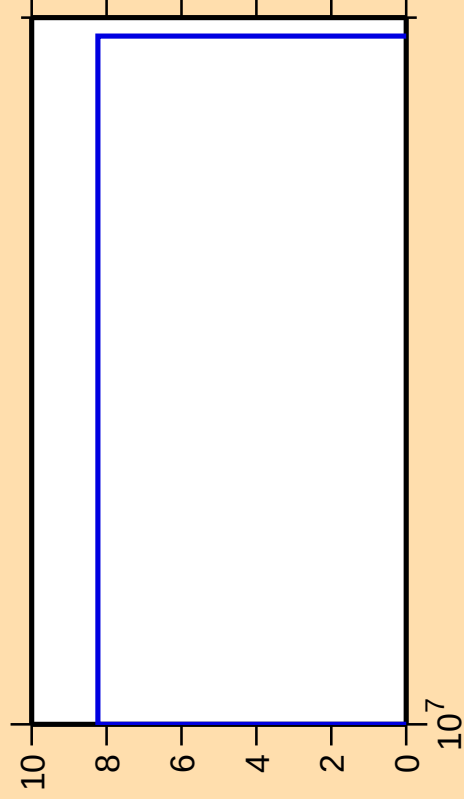
\Delta\sigma/\sigma vs. E for ^{229}\text{Th}(n,\text{nt})
