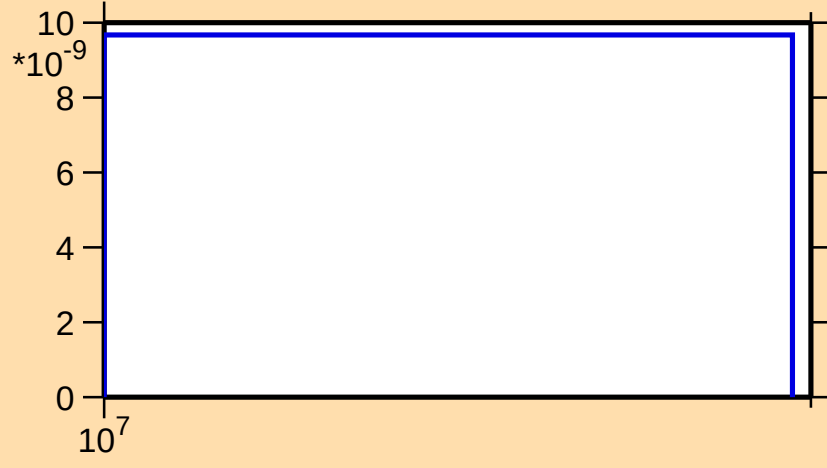
\sigma vs. E for ^{229}\text{Th}(n,\text{nt})
