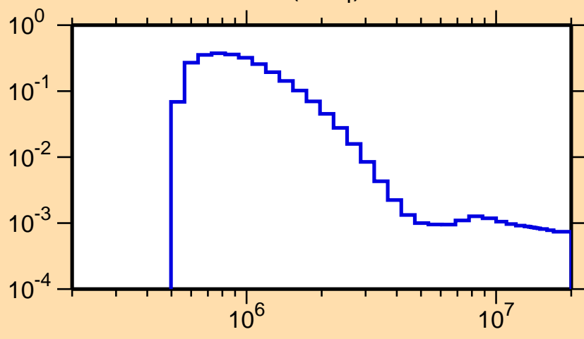
\sigma vs. E for ^{230}\text{Th}(n,n_4)
