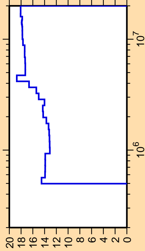
\Delta\sigma/\sigma vs. E for ^{230}\text{Th}(n,n_4)
