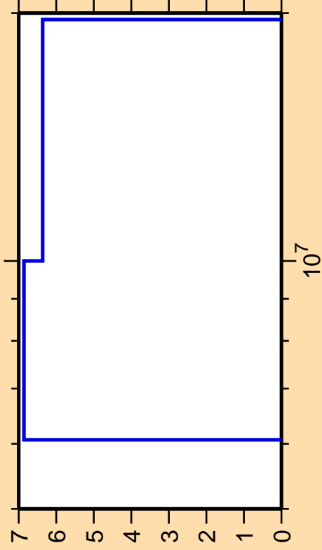
\Delta\sigma/\sigma vs. E for ^{230}\text{Th}(n,p)
