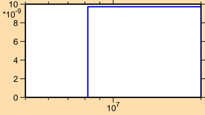
\sigma vs. E for ^{230}\text{Th}(n,2n\alpha)
