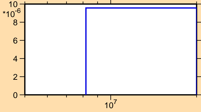
\sigma vs. E for ^{230}\text{Th}(n,t)
