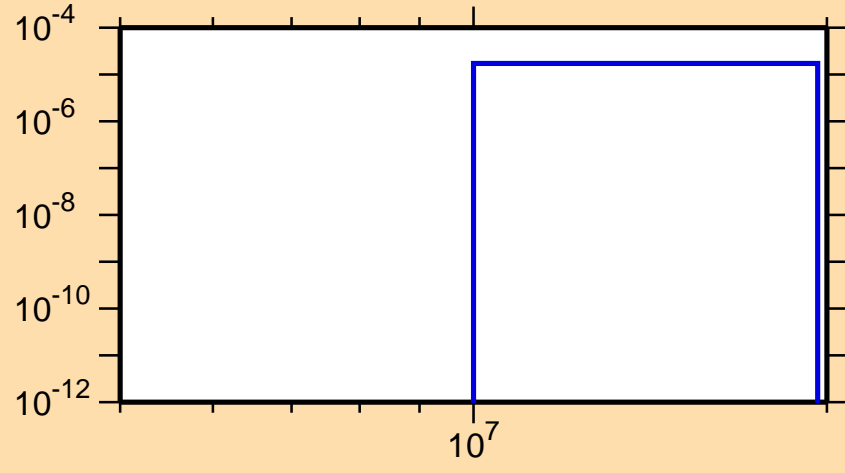
\sigma vs. E for ^{232}\text{Th}(n,d)
