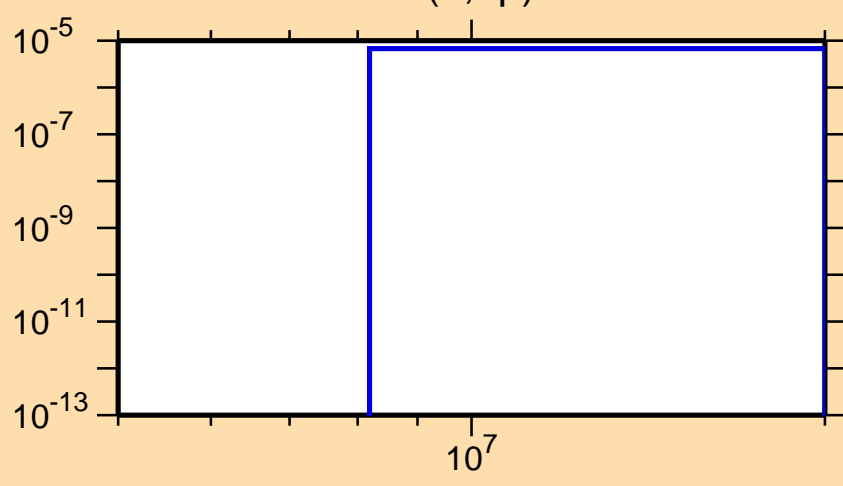
\sigma vs. E for ^{232}\text{Th}(n,np)
