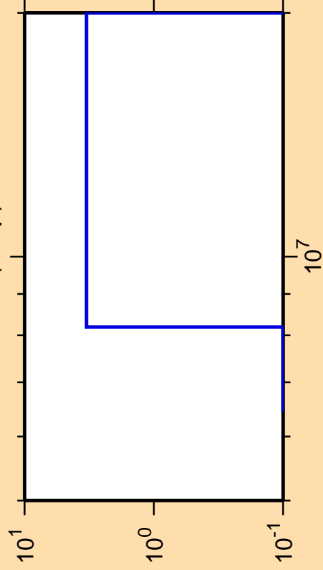
\Delta\sigma/\sigma vs. E for ^{232}\text{Th}(n,np)
