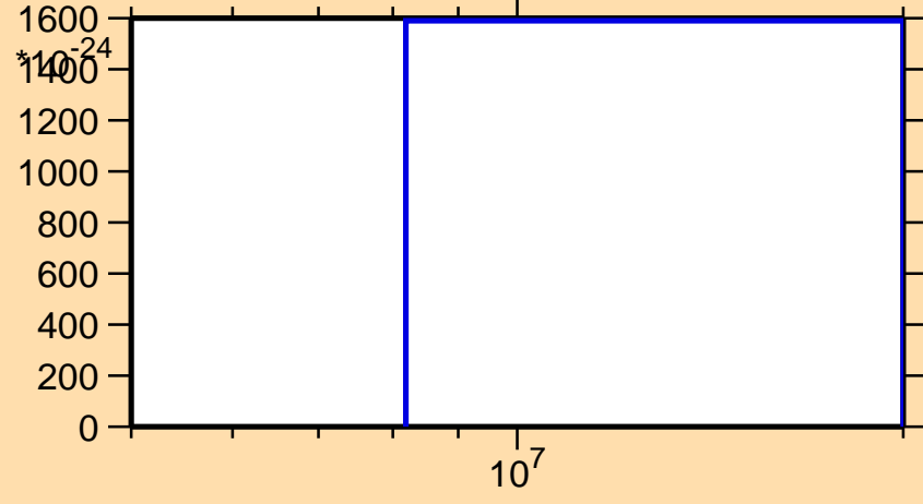
\sigma vs. E for ^{232}\text{Th} (mt 42)
