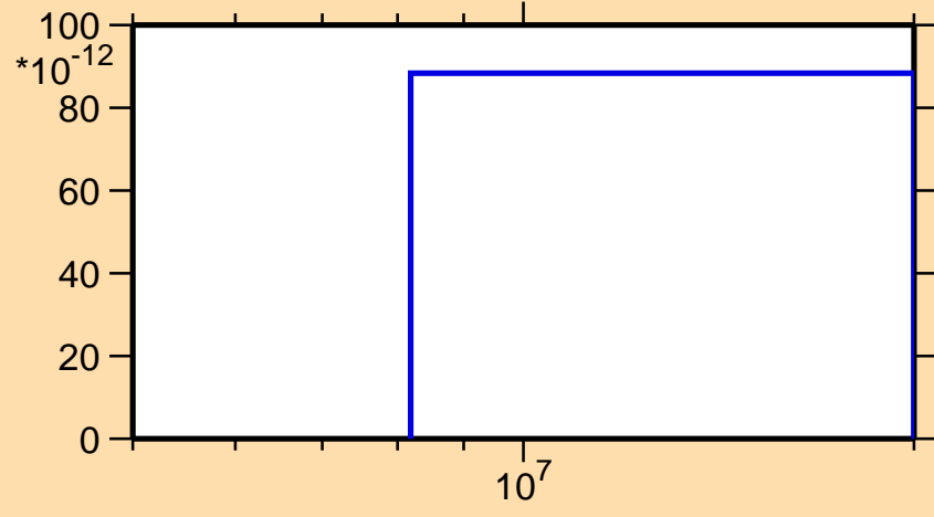
\sigma vs. E for ^{232}\text{Th}(n,\text{nd})
