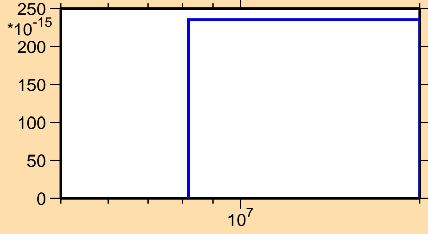
\sigma vs. E for ^{232}\text{Th}(n,3n\alpha)
