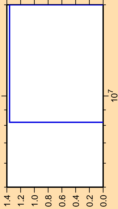
\Delta\sigma/\sigma vs. E for ^{232}\text{Th}(n,t)
