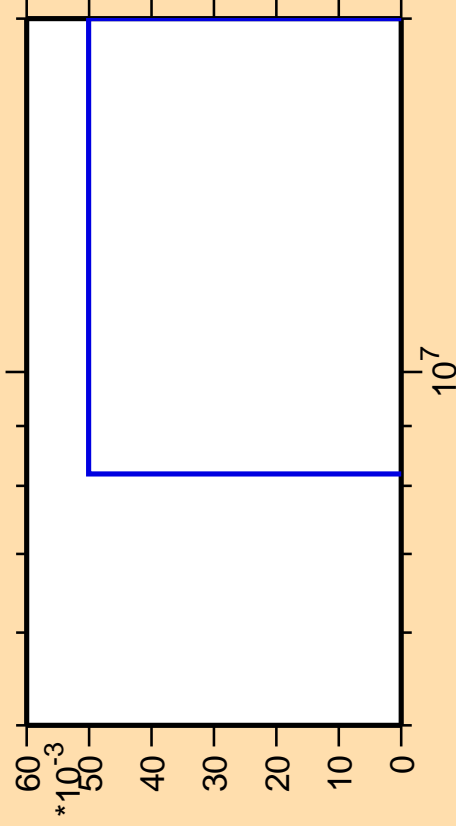
\Delta\sigma/\sigma vs. E for ^{232}\text{Th}(n,3n\alpha)
