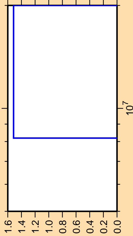
\Delta\sigma/\sigma vs. E for ^{232}\text{Th}(n,d)
