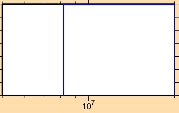
\sigma vs. E for ^{232}\text{Th}(n,d)
