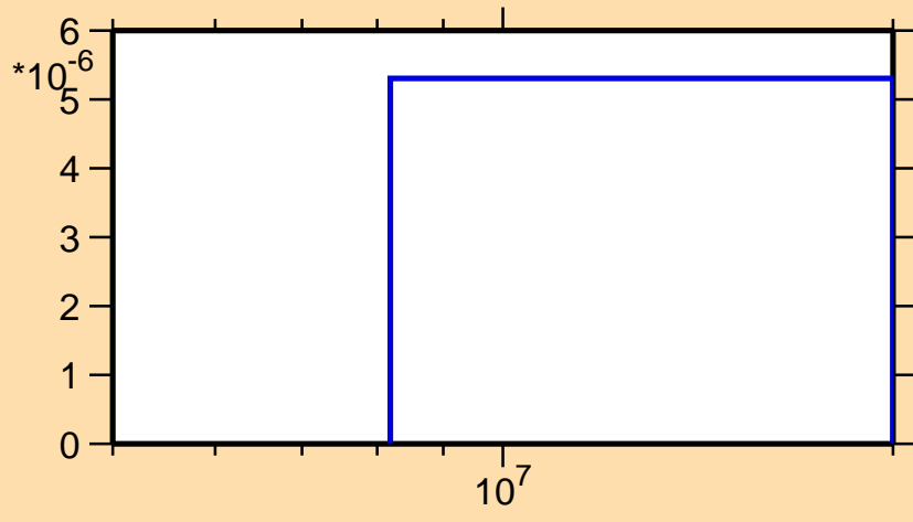
\sigma vs. E for ^{232}\text{Th}(n,t)
