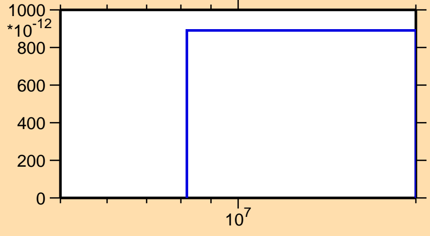
\sigma vs. E for ^{232}\text{Th}(n,2n\alpha)
