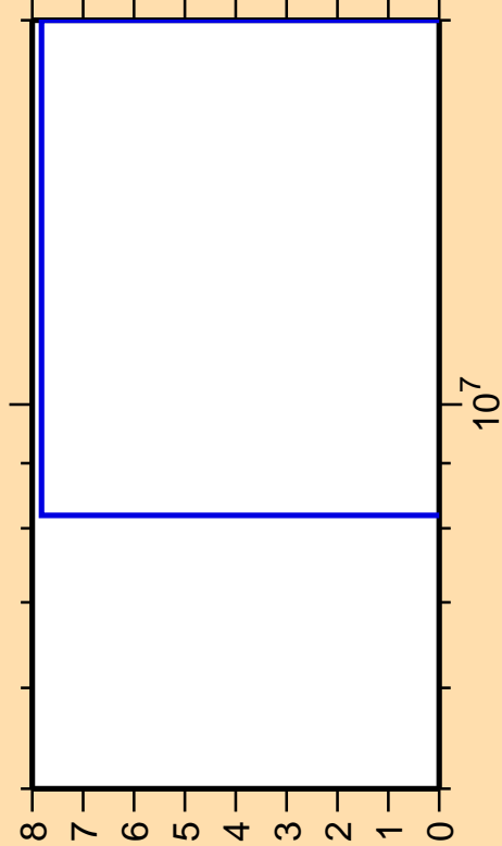
\Delta\sigma/\sigma vs. E for ^{232}\text{Th}(n,2n\alpha)
