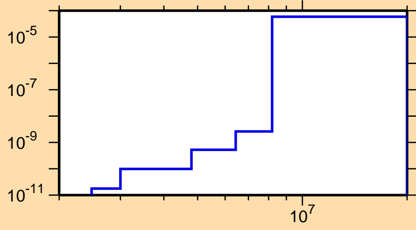
\sigma vs. E for ^{232}\text{Th}(n,\alpha)
