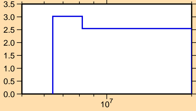
\Delta\sigma/\sigma vs. E for ^{232}\text{Th}(n,p)
