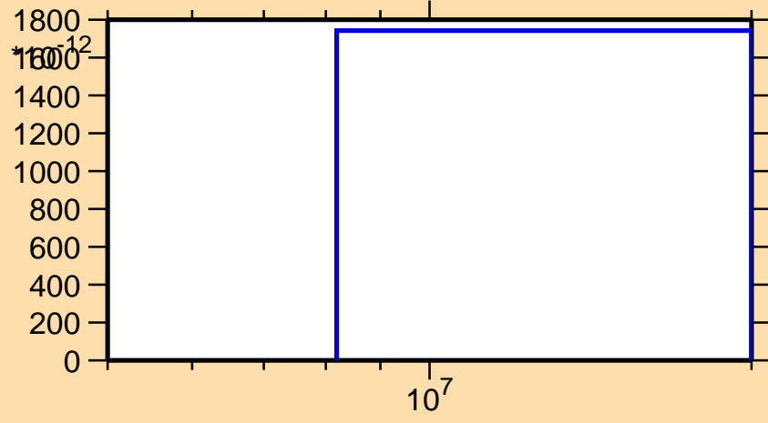
\sigma vs. E for ^{232}\text{Th}(n,nt)
