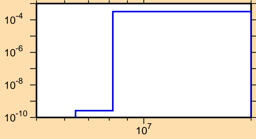
\sigma vs. E for ^{232}\text{Th}(n,p)
