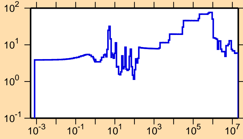
\Delta\sigma/\sigma vs. E for ^{233}\text{Th}(n,el.)
