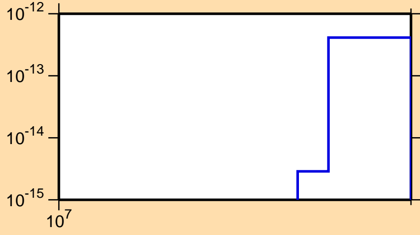
\sigma vs. E for ^{233}\text{Th}(n,\text{He3})
