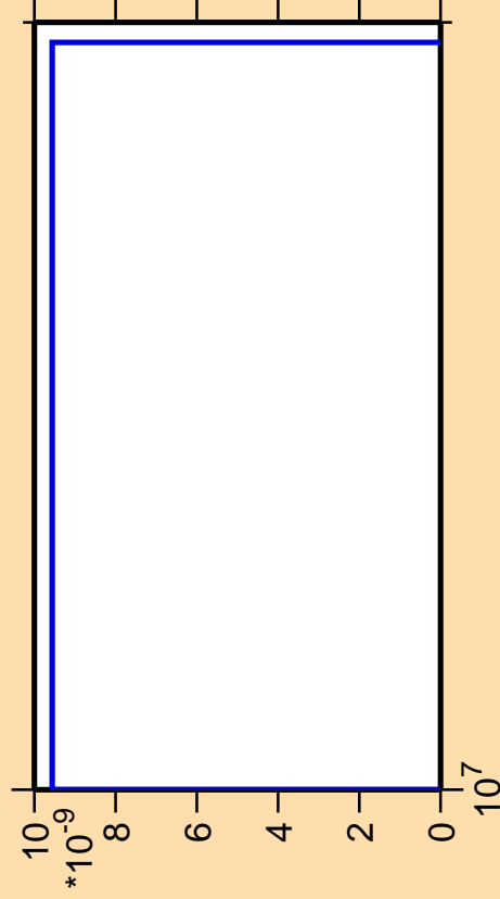
\Delta\sigma/\sigma vs. E for ^{233}\text{Th} (mt 42)
