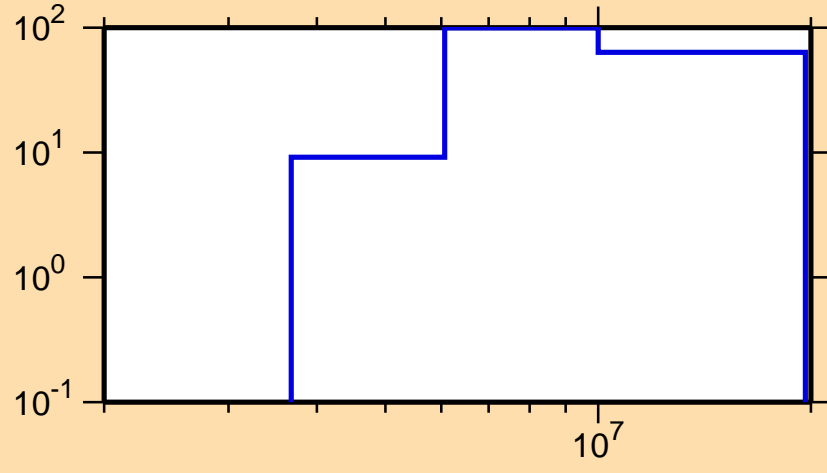
\Delta\sigma/\sigma vs. E for ^{233}\text{Th}(n,p)
