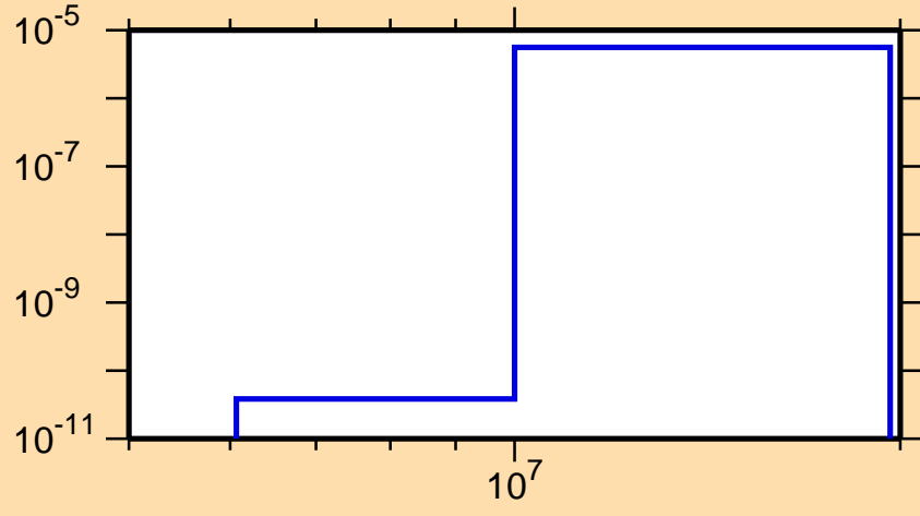
\sigma vs. E for ^{233}\text{Th}(n,\alpha)
