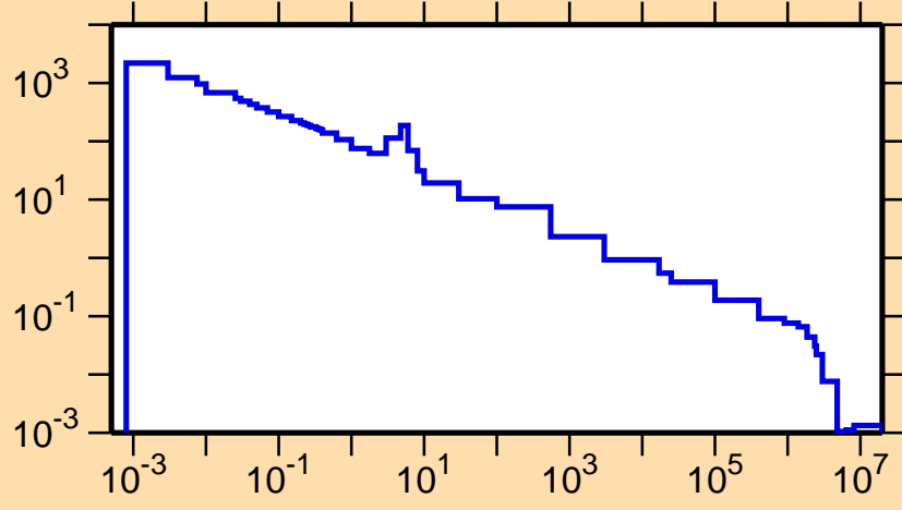
\sigma vs. E for ^{233}\text{Th}(n,\gamma)
