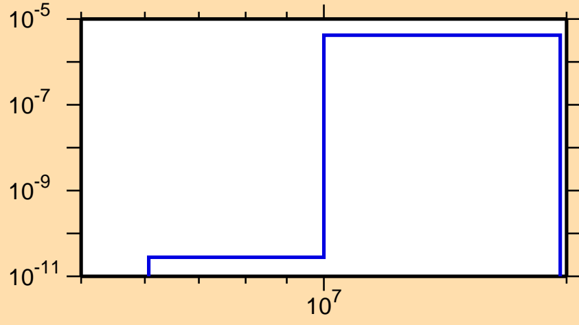
\sigma vs. E for ^{234}\text{Th}(n,n\alpha)
