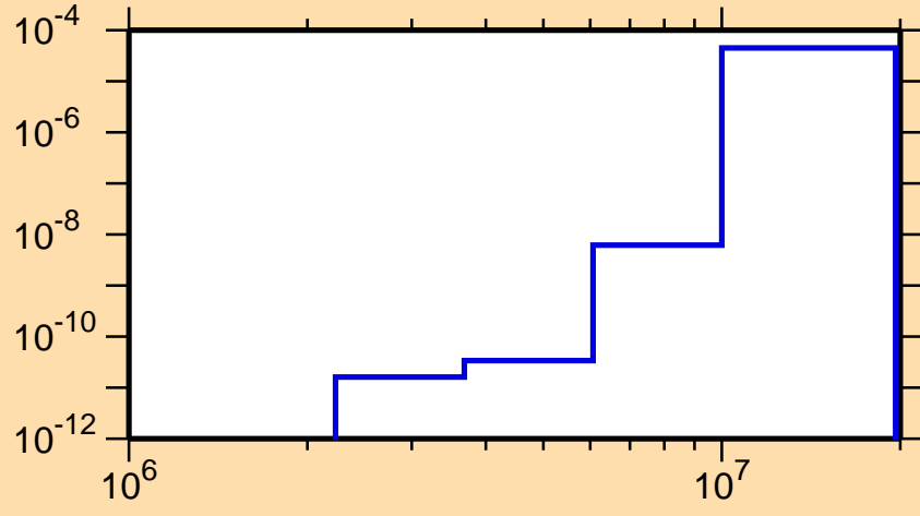
\sigma vs. E for ^{234}\text{Th}(n,\alpha)
