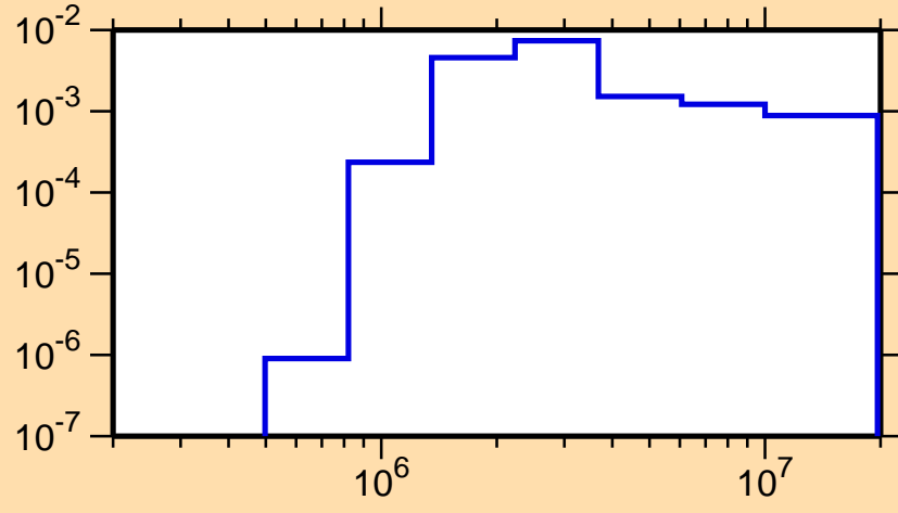
\sigma vs. E for ^{234}\text{Th}(n,n_4)
