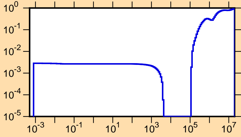
\mu vs. E for ^{236}\text{Th}(\text{mt251})
