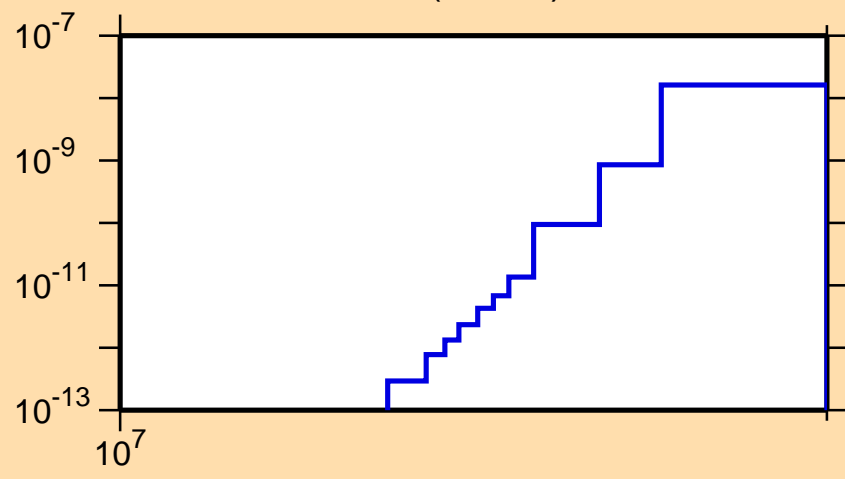
\sigma vs. E for ^{236}\text{Th}(n,2n\alpha)
