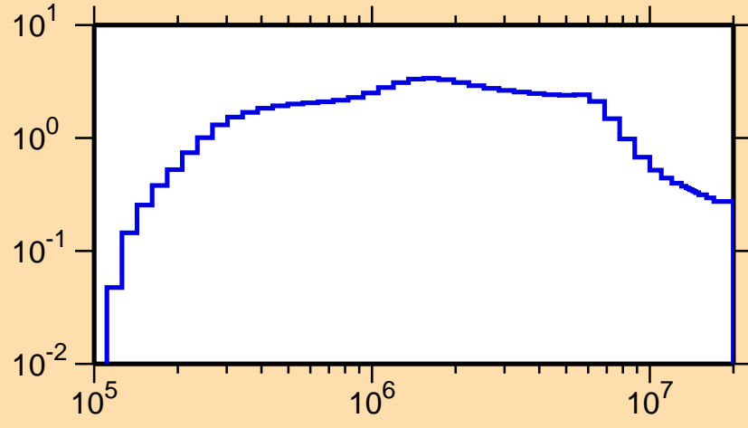
\sigma vs. E for ^{236}\text{Th}(n,\text{inel.})
