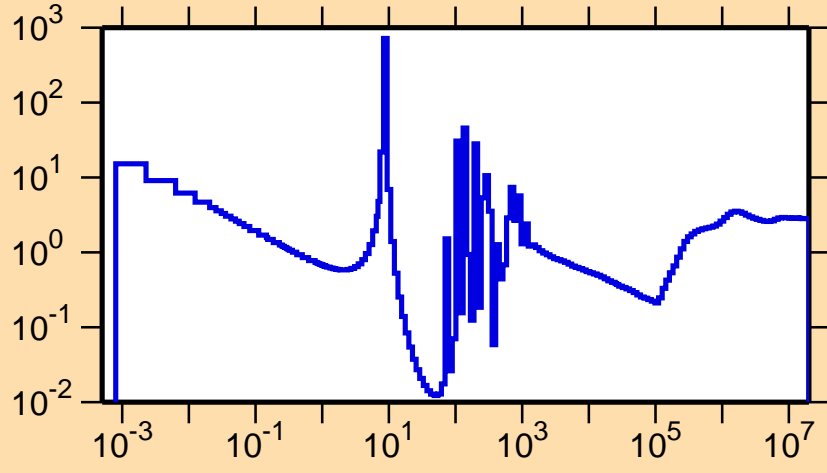
\sigma vs. E for ^{236}\text{Th}(n,\text{nonel.})
