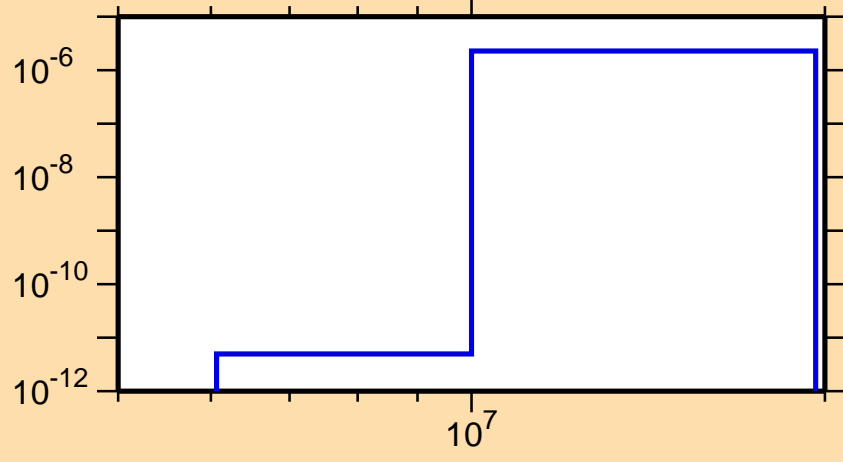
\sigma vs. E for ^{236}\text{Th}(n,\alpha)
