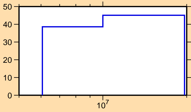
\Delta\sigma/\sigma vs. E for ^{236}\text{Th}(n,el.)
