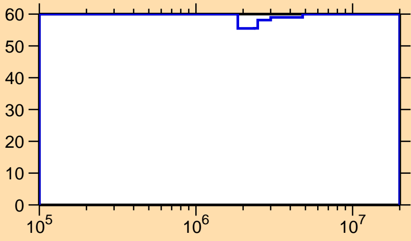
\Delta\sigma/\sigma vs. E for ^{236}\text{Th}(n,\text{inel.})
