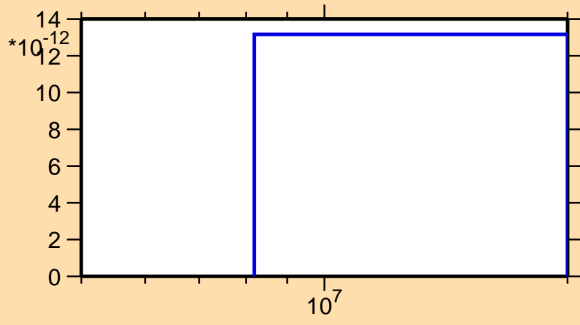
\sigma vs. E for ^{236}\text{Th}(n,2np)
