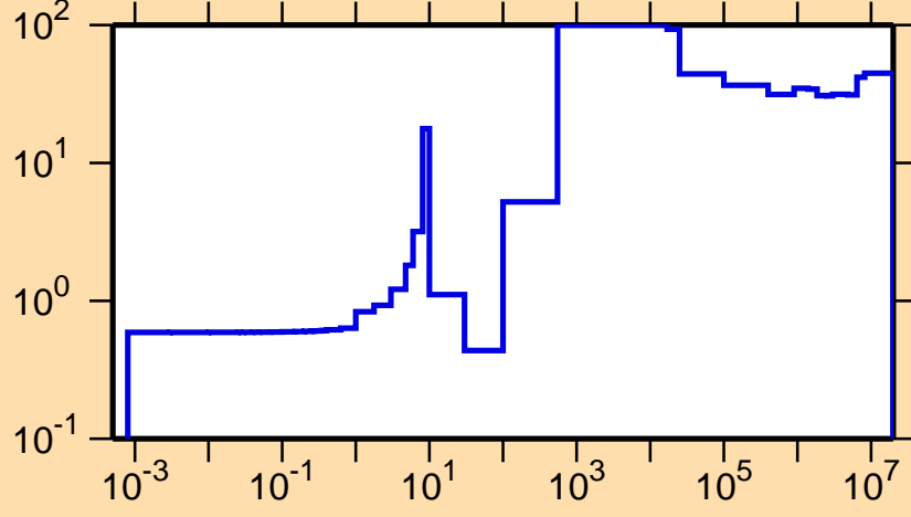
\Delta\sigma/\sigma vs. E for ^{236}\text{Th}(n,el.)
