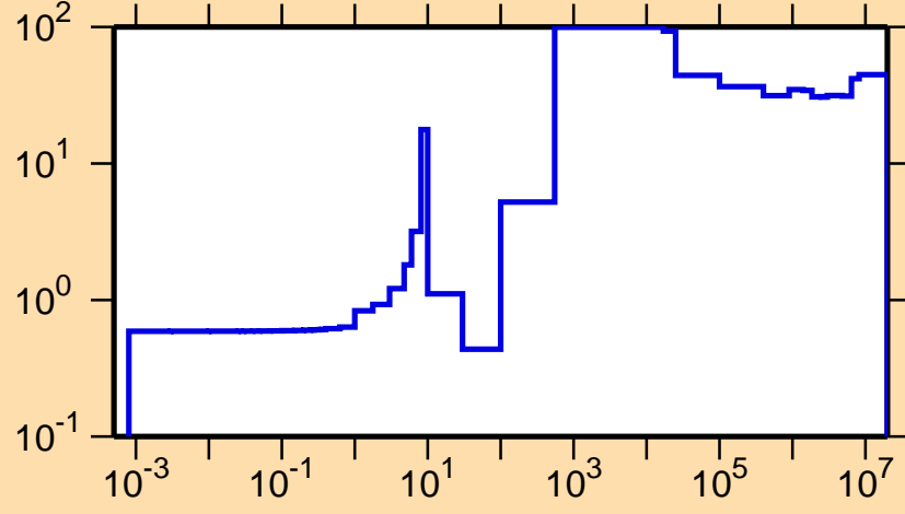
\Delta\sigma/\sigma vs. E for ^{236}\text{Th}(n,\text{el.})
