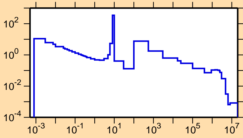
\sigma vs. E for ^{236}\text{Th}(n,\gamma)
