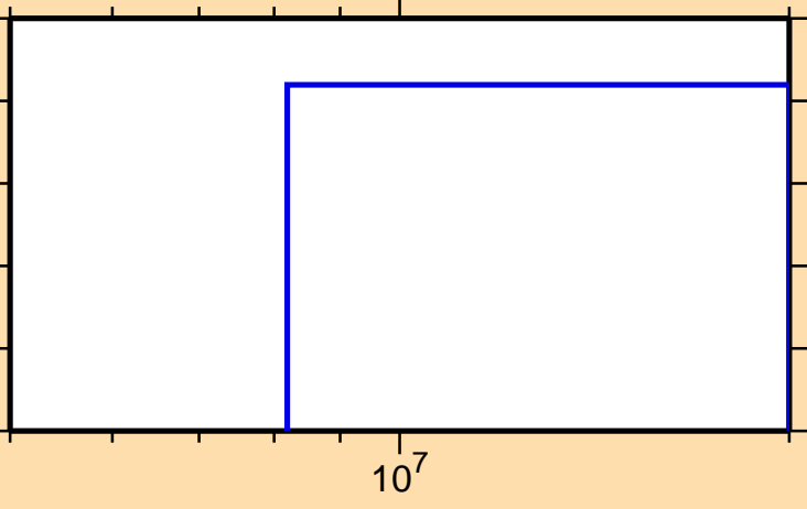
\sigma vs. E for ^{236}\text{Th}(n,t)
