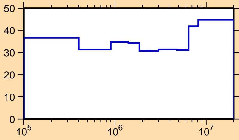
\Delta\sigma/\sigma vs. E for ^{236}\text{Th}(n,\text{el.})
