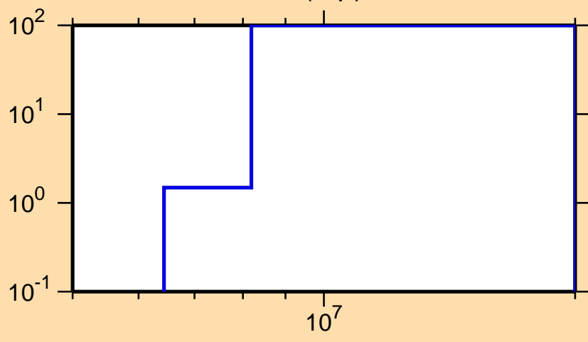
\Delta\sigma/\sigma vs. E for ^{236}\text{Th}(n,p)
