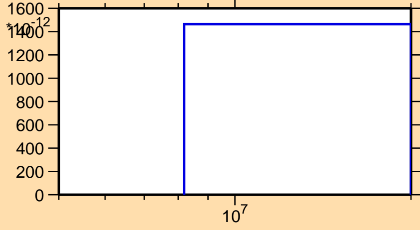
\sigma vs. E for ^{236}\text{Th}(n,nt)
