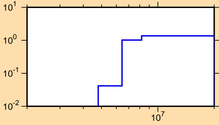
\sigma vs. E for ^{236}\text{Th}(n,2n)
