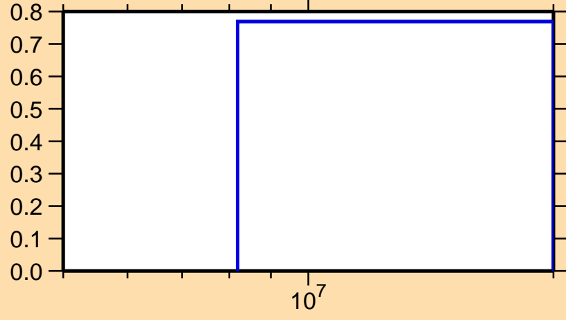
\sigma vs. E for ^{236}\text{Th}(n,3n)
