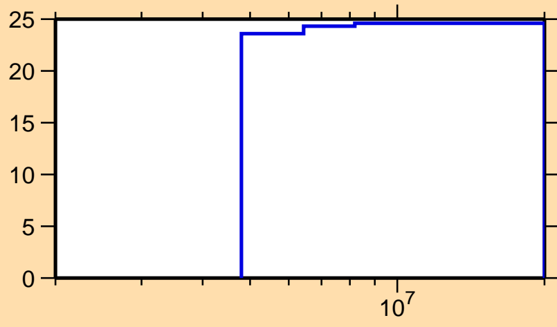
\Delta\sigma/\sigma vs. E for ^{236}\text{Th}(n,\text{tot.})
