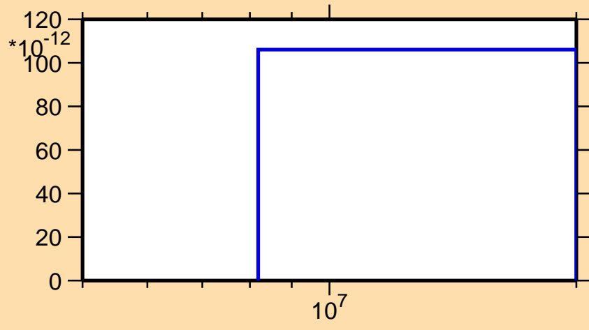
\sigma vs. E for ^{236}\text{Th}(n,\text{nd})
