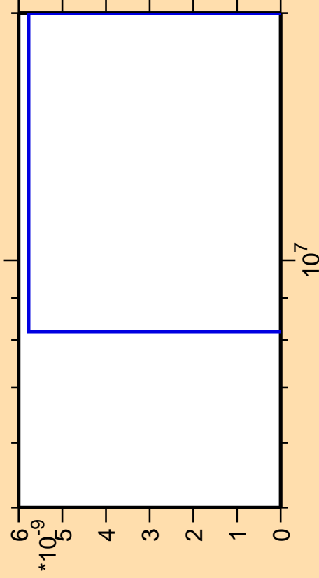
\Delta\sigma/\sigma vs. E for ^{236}\text{Th} (mt 42)
