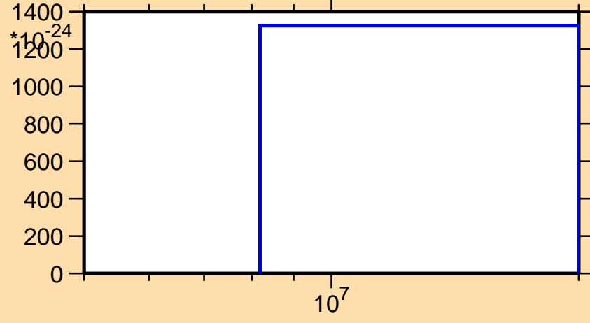
\sigma vs. E for ^{236}\text{Th} (mt 42)
