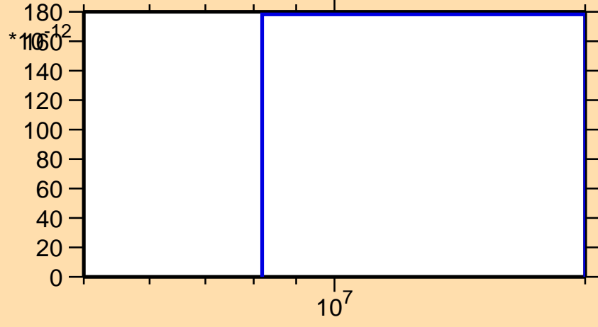
\sigma vs. E for ^{236}\text{Th}(n,2n\alpha)
