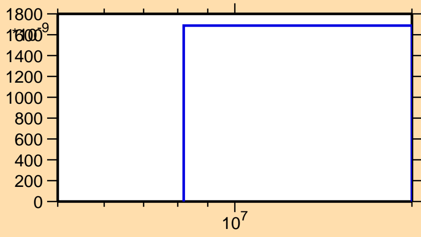
\sigma vs. E for ^{236}\text{Th}(n,np)
