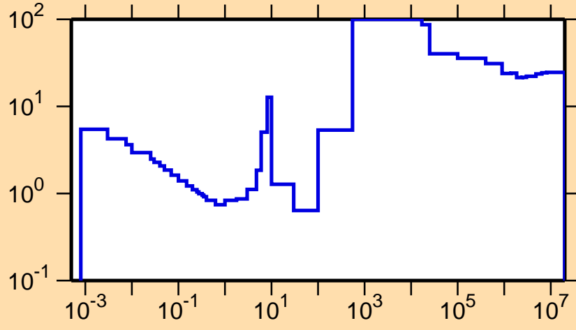
\Delta\sigma/\sigma vs. E for ^{236}\text{Th}(n,\text{tot.})
