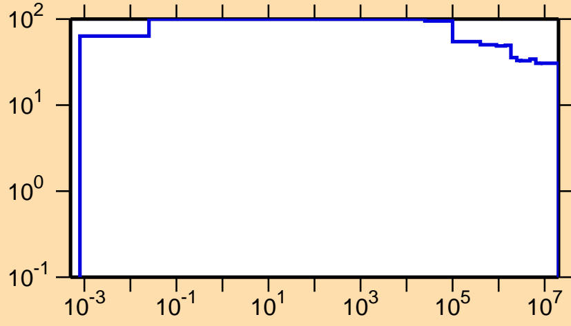
\Delta\sigma/\sigma vs. E for ^{236}\text{Th}(n,\text{nonel.})
