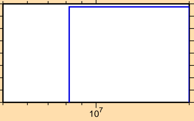
\sigma vs. E for ^{236}\text{Th}(n,d)
