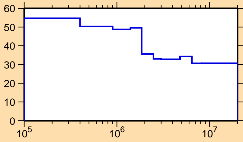
\Delta\sigma/\sigma vs. E for ^{236}\text{Th}(n,\text{nonel.})
