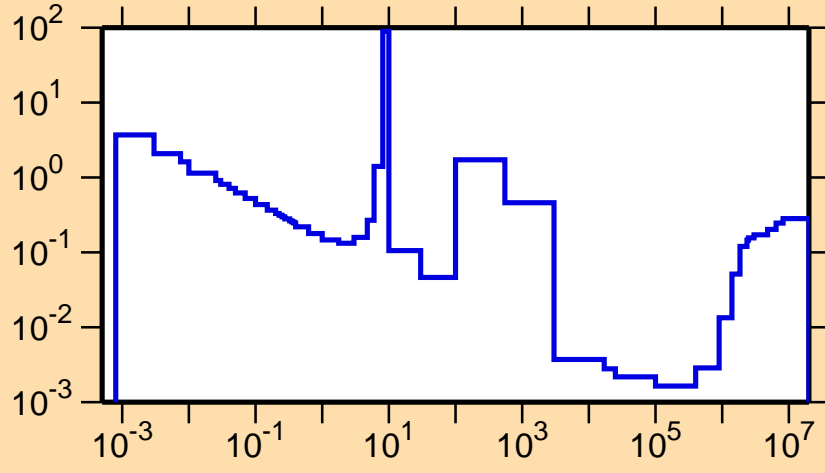
\sigma vs. E for ^{236}\text{Th}(n,f)
