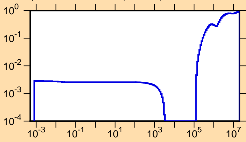
\mu vs. E for ^{237}\text{Th}(\text{mt251})
