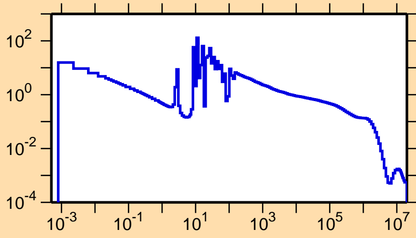
\sigma vs. E for ^{237}\text{Th}(n,\gamma)
