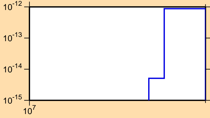
\sigma vs. E for ^{237}\text{Th}(n,3n\alpha)
