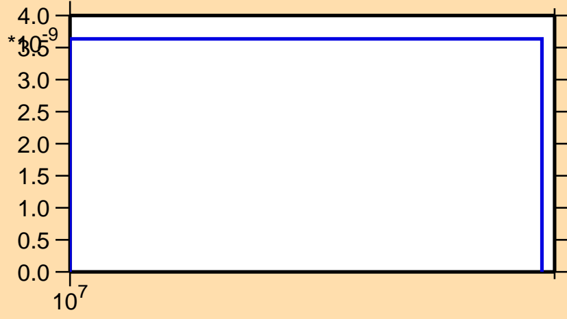
\sigma vs. E for ^{237}\text{Th}(n,2n\alpha)
