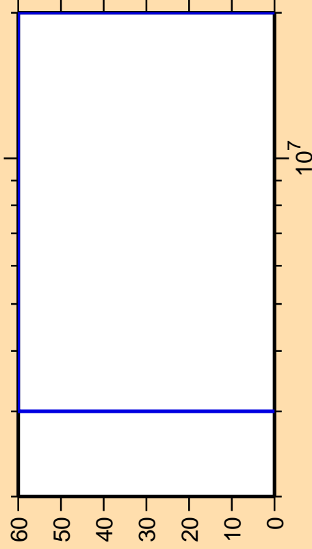
\Delta\sigma/\sigma vs. E for ^{237}\text{Th}(n,n\text{cont.})
