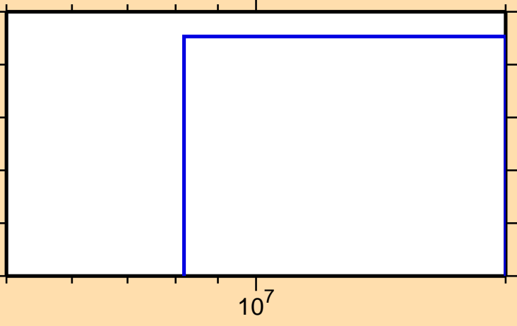
\sigma vs. E for ^{237}\text{Th}(n,nt)
