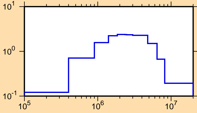
\sigma vs. E for ^{237}\text{Th}(n,n\text{cont.})
