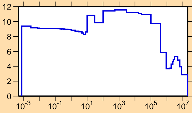
\sigma vs. E for ^{237}\text{Th}(n,\text{el.})
