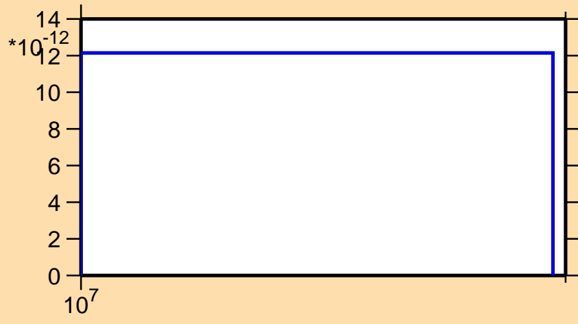
\sigma vs. E for ^{238}\text{Th}(n,2np)
