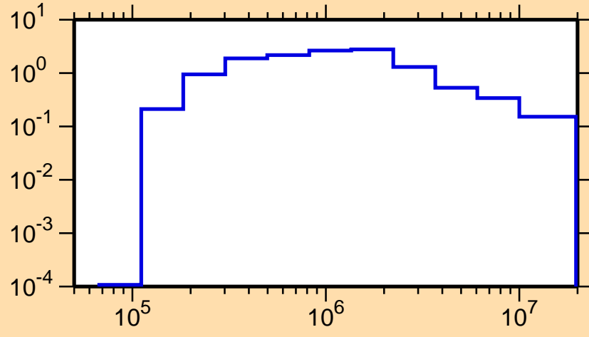
\sigma vs. E for ^{238}\text{Th}(n,n_1)
