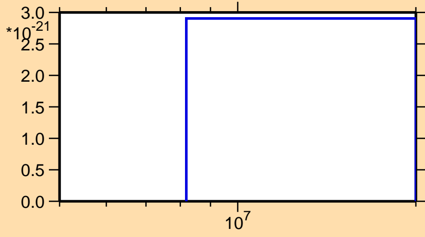
\sigma vs. E for ^{238}\text{Th} (mt 42)
