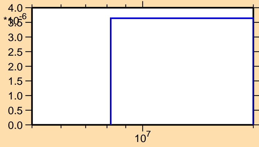
\sigma vs. E for ^{238}\text{Th}(n,t)
