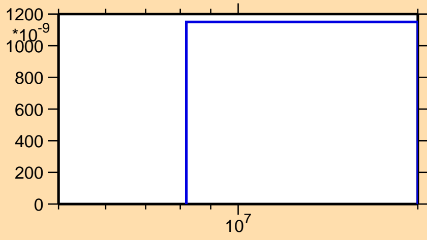
\sigma vs. E for ^{238}\text{Th}(n,np)
