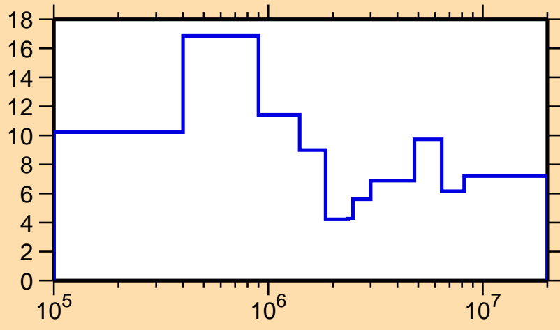
\Delta\sigma/\sigma vs. E for ^{238}\text{Th}(n,\text{tot.})
