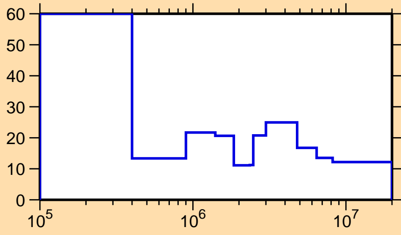
\Delta\sigma/\sigma vs. E for ^{238}\text{Th}(n,\text{nonel.})
