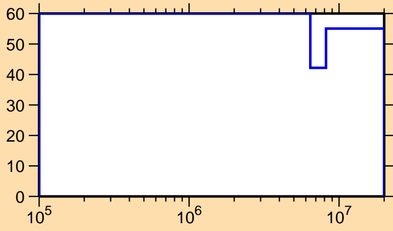
\Delta\sigma/\sigma vs. E for ^{238}\text{Th}(n,\text{inel.})
