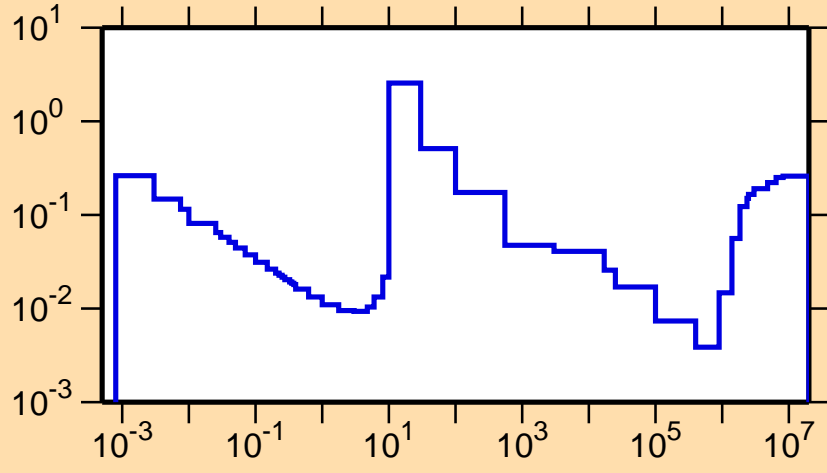
\sigma vs. E for ^{238}\text{Th}(n,f)
