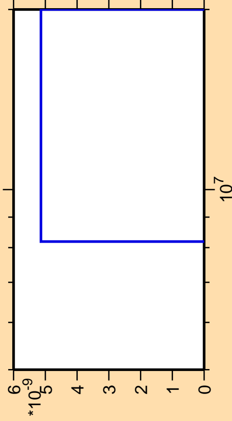
\Delta\sigma/\sigma vs. E for ^{238}\text{Th} (mt 42)
