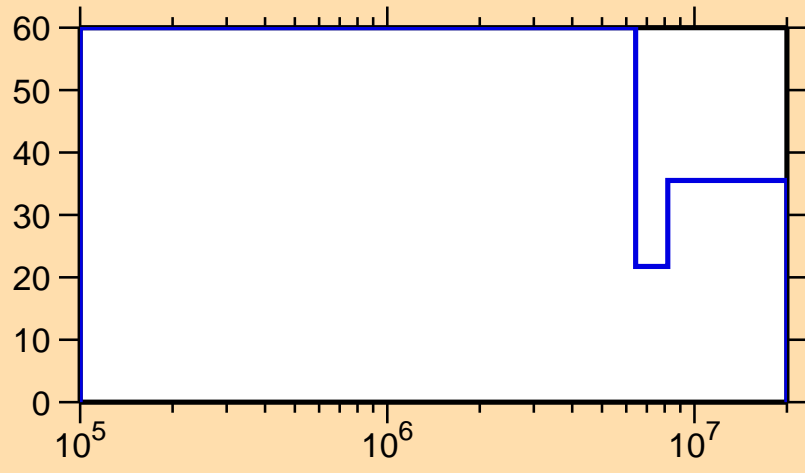
\Delta\sigma/\sigma vs. E for ^{238}\text{Th}(n,n\text{cont.})
