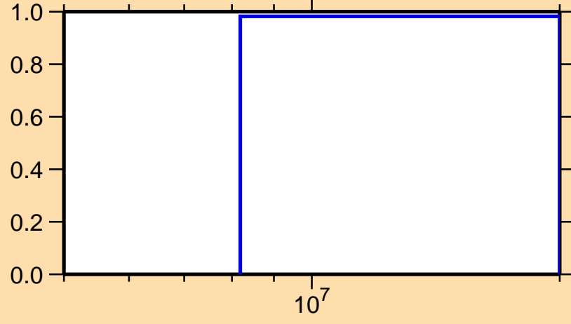
\sigma vs. E for ^{238}\text{Th}(n,3n)
