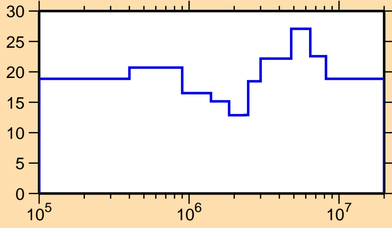
\Delta\sigma/\sigma vs. E for ^{238}\text{Th}(n,\text{el.})
