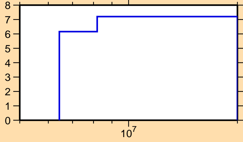
\Delta\sigma/\sigma vs. E for ^{238}\text{Th}(n,\text{tot.})
