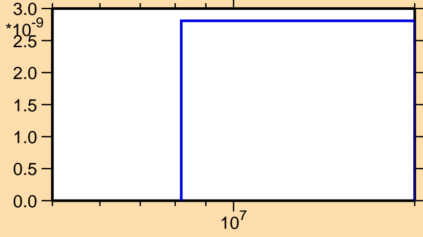
\sigma vs. E for ^{238}\text{Th}(n,nt)
