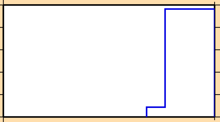
\sigma vs. E for ^{44}\text{Ti} (mt 45)
