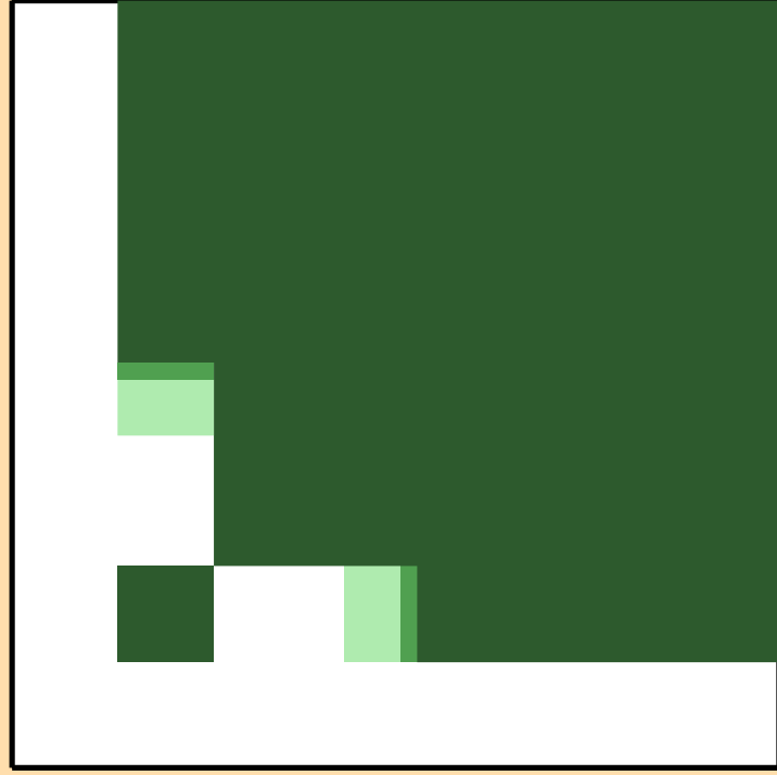
\sigma vs. E for ^{44}\text{Ti}(n,pd)
