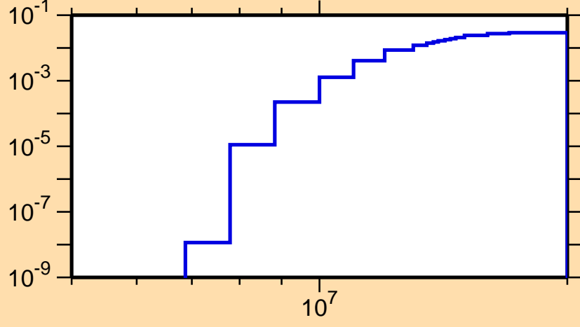
\sigma vs. E for ^{44}\text{Ti}(n,d)
