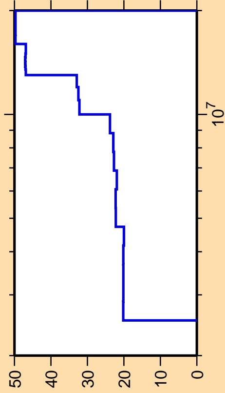
\Delta\sigma/\sigma vs. E for ^{44}\text{Ti}(n,n_4)
