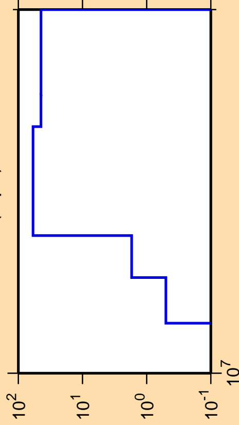
\Delta\sigma/\sigma vs. E for ^{44}\text{Ti}(n,pd)
