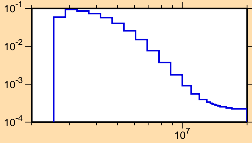
\sigma vs. E for ^{44}\text{Ti}(n,n_4)
