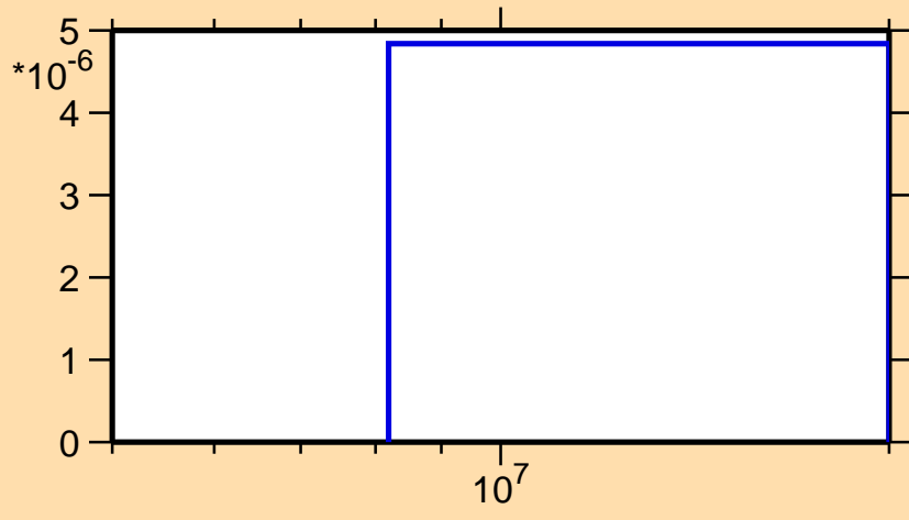
\sigma vs. E for ^{44}\text{Ti}(n,t)
