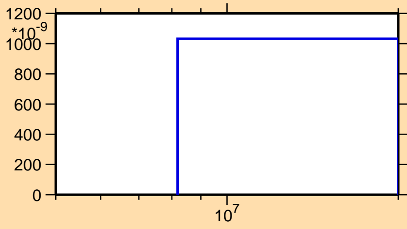
\sigma vs. E for ^{44}\text{Ti}(n,2n)
