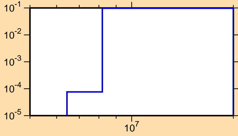
\sigma vs. E for ^{44}\text{Ti}(n,n\alpha)
