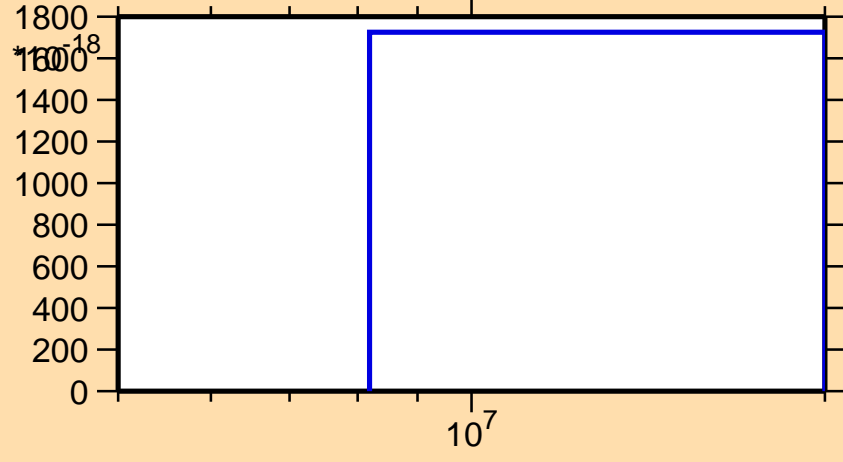
\sigma vs. E for ^{44}\text{Ti}(n,nd)
