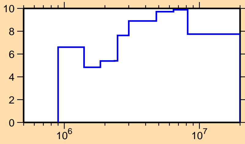
\Delta\sigma/\sigma vs. E for ^{44}\text{Ti}(n,\text{el.})
