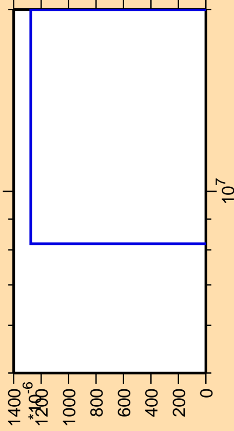
\Delta\sigma/\sigma vs. E for ^{44}\text{Ti}(n,nd)
