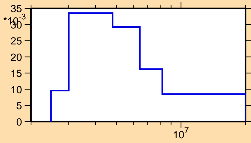
\sigma vs. E for ^{44}\text{Ti}(n,n_3)
