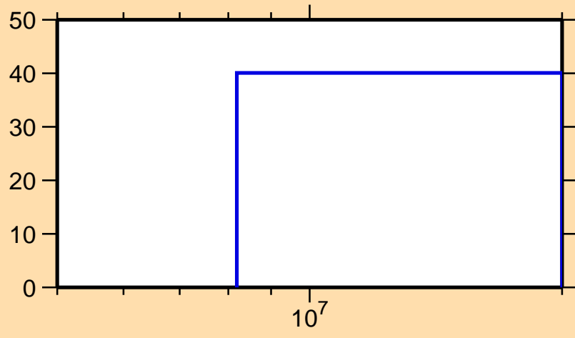
\Delta\sigma/\sigma vs. E for ^{44}\text{Ti}(n,2n)
