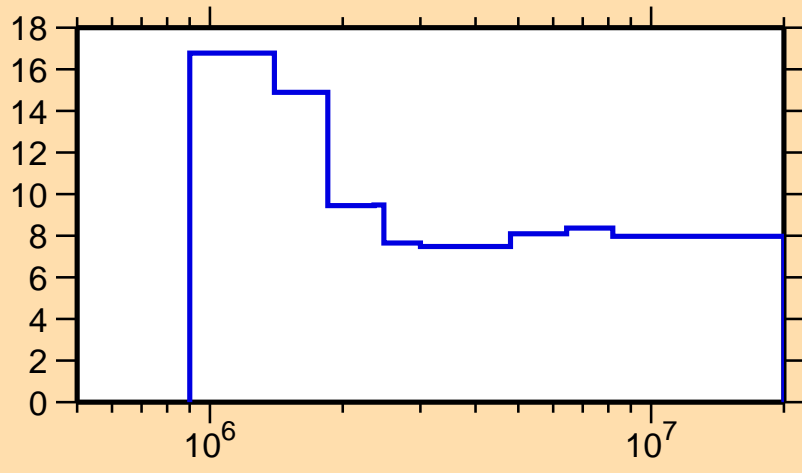
\Delta\sigma/\sigma vs. E for ^{44}\text{Ti}(n,\text{nonel.})
