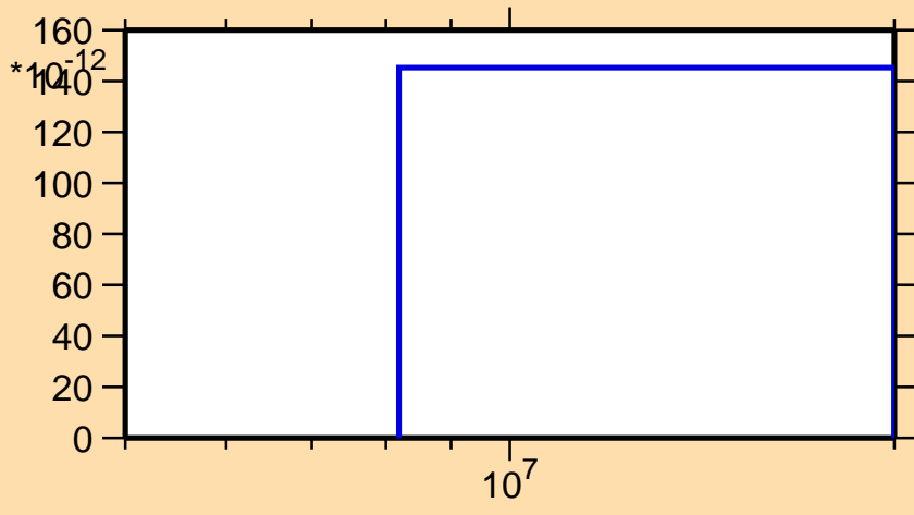
\sigma vs. E for ^{44}\text{Ti}(n,\text{pt})
