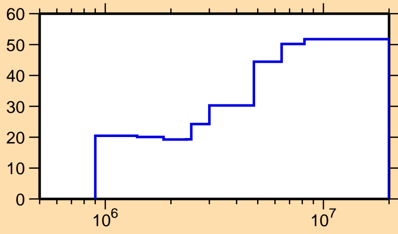
\Delta\sigma/\sigma vs. E for ^{44}\text{Ti}(n,n_1)
