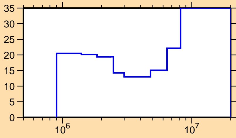
\Delta\sigma/\sigma vs. E for ^{44}\text{Ti}(n,\text{inel.})
