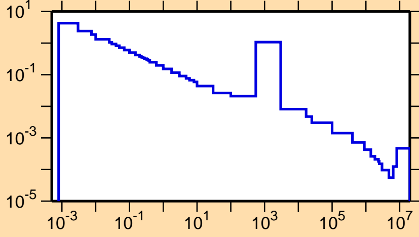
\sigma vs. E for ^{44}\text{Ti}(n,\gamma)
