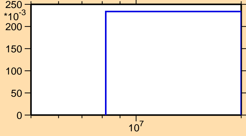
\sigma vs. E for ^{44}\text{Ti}(n,np)
