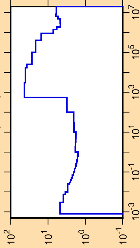
\Delta\sigma/\sigma vs. E for ^{44}\text{Ti}(n,\text{tot.})
