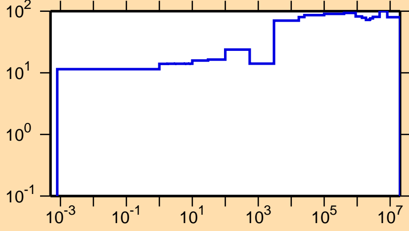
\Delta\sigma/\sigma vs. E for ^{44}\text{Ti}(n,\gamma)
