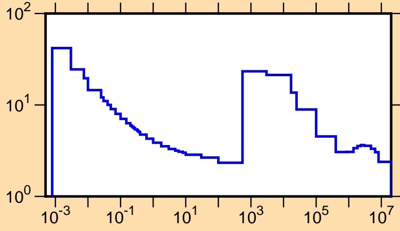
\sigma vs. E for ^{44}\text{Ti}(n,\text{tot.})
