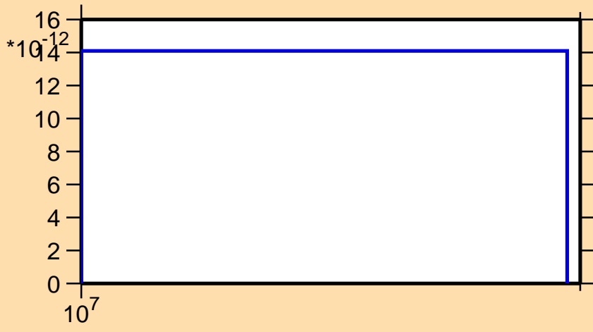
\sigma vs. E for ^{45}\text{Ti} (mt 34)
