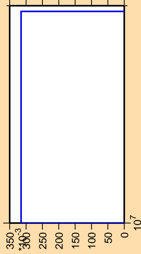
\Delta\sigma/\sigma vs. E for ^{45}\text{Ti} (mt 45)
