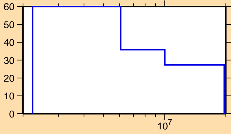
\Delta\sigma/\sigma vs. E for ^{45}\text{Ti}(n,n\text{cont.})
