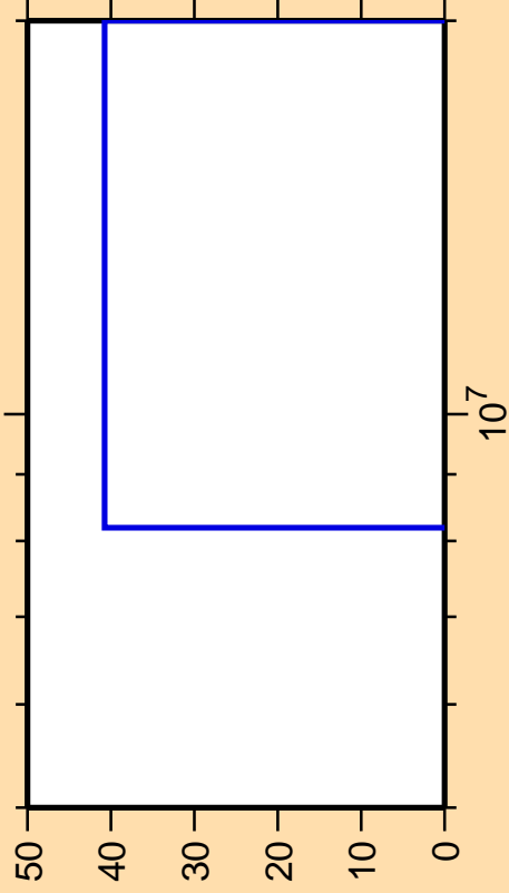
\Delta\sigma/\sigma vs. E for ^{45}\text{Ti}(n,t)
