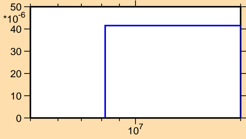
\sigma vs. E for ^{45}\text{Ti}(n,t)
