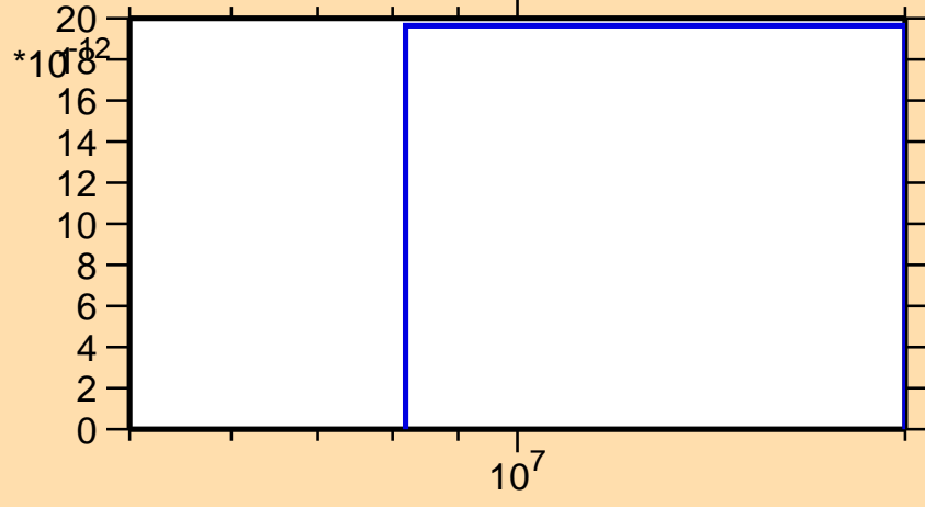
\sigma vs. E for ^{45}\text{Ti} (mt 34)
