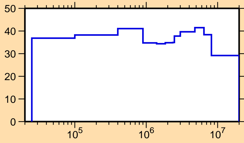
\Delta\sigma/\sigma vs. E for ^{45}\text{Ti}(n,n_1)
