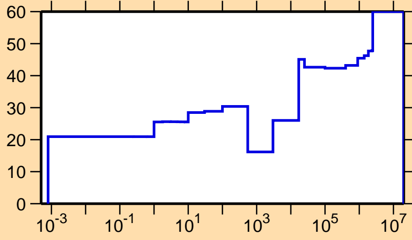
\Delta\sigma/\sigma vs. E for ^{45}\text{Ti}(n,\gamma)
