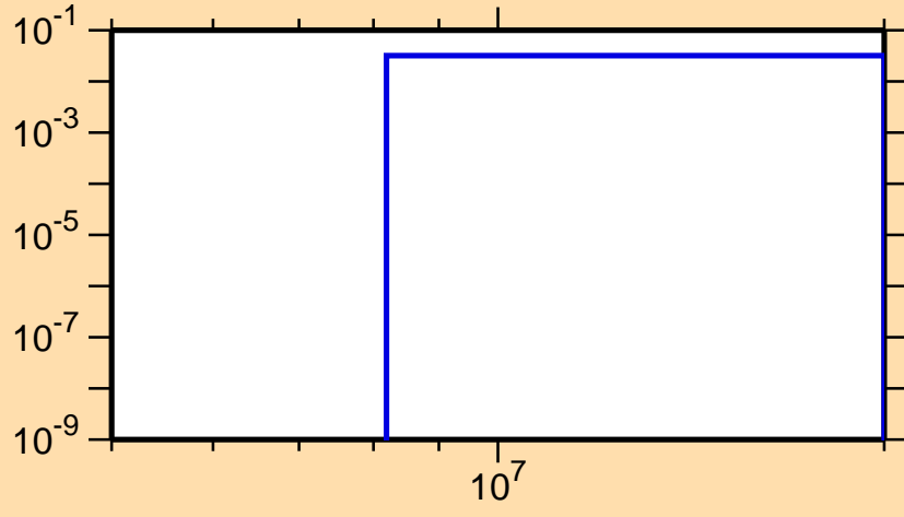
\sigma vs. E for ^{45}\text{Ti}(n,n\alpha)
