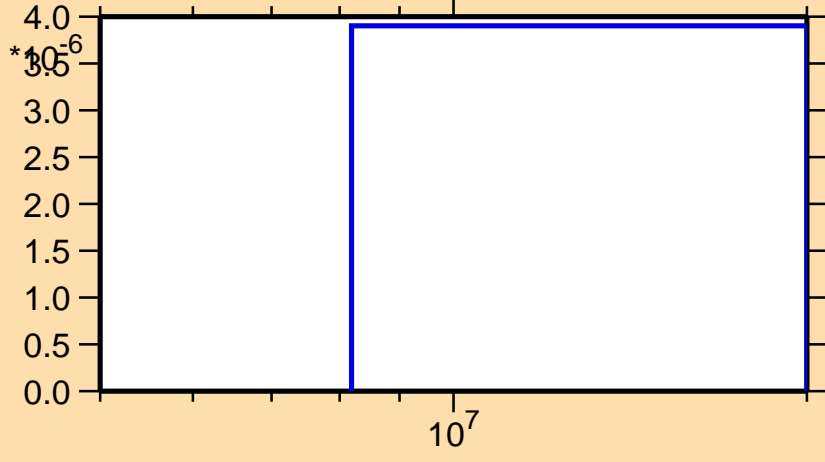
\sigma vs. E for ^{45}\text{Ti}(n,\text{pd})
