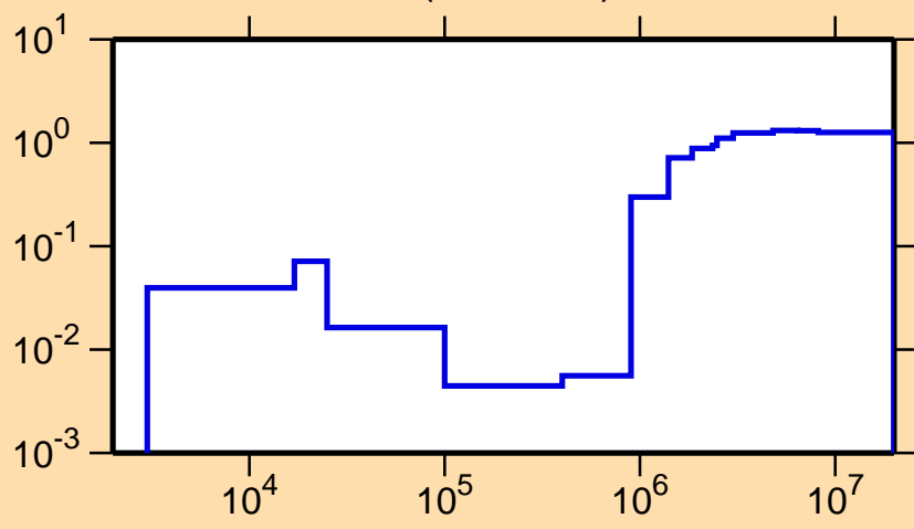
\sigma vs. E for ^{48}\text{Ti}(n,\text{nonel.})
