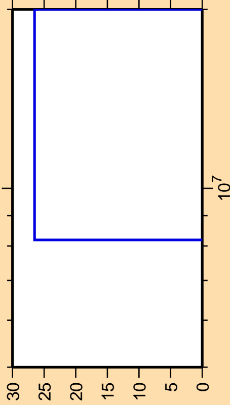
\Delta\sigma/\sigma vs. E for ^{48}\text{Ti}(n,n_1)
