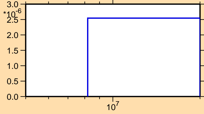
\sigma vs. E for ^{48}\text{Ti}(n,3n)
