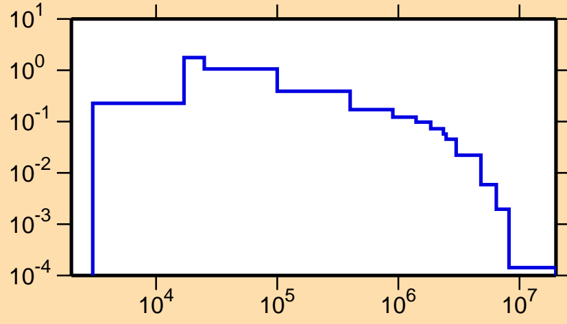
\sigma vs. E for ^{48}\text{Ti}(n,n_4)
