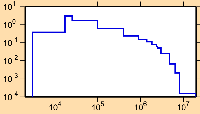
\sigma vs. E for ^{48}\text{Ti}(n,n_2)
