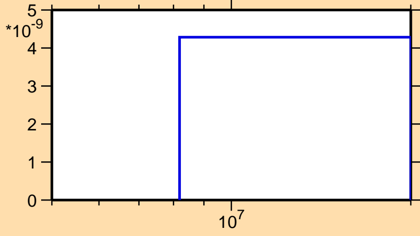
\sigma vs. E for ^{48}\text{Ti}(n,pd)
