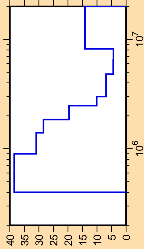
\Delta\sigma/\sigma vs. E for ^{48}\text{Ti}(n,\text{ncont.})
