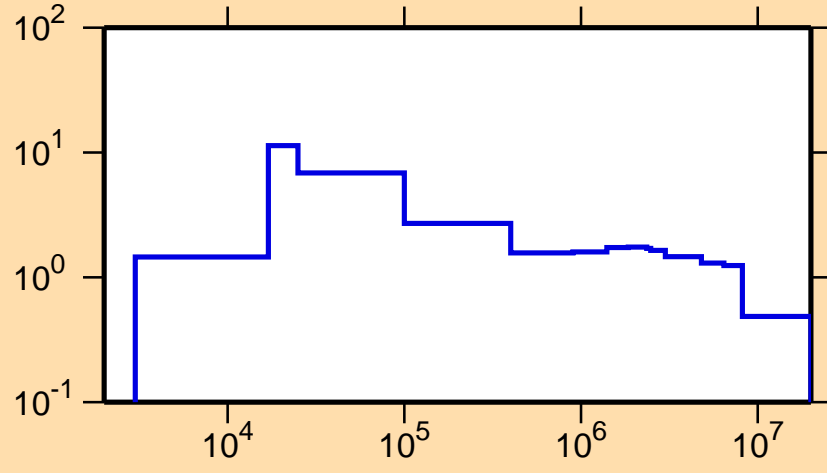
\sigma vs. E for ^{48}\text{Ti}(n,\text{inel.})
