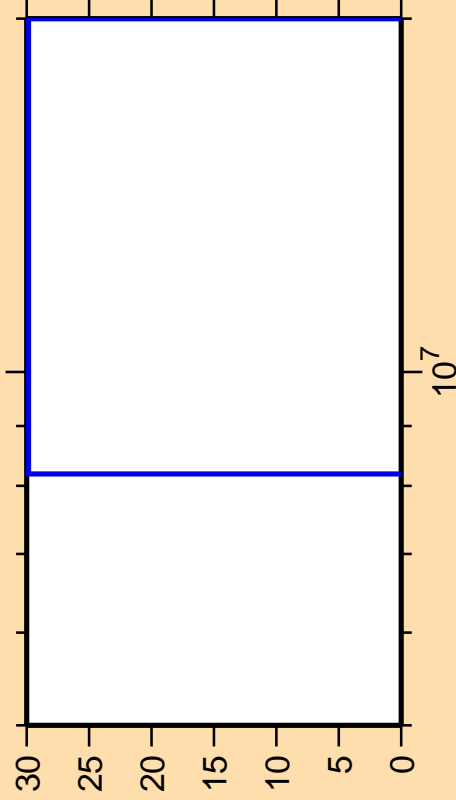
\Delta\sigma/\sigma vs. E for ^{48}\text{Ti}(n,nd)
