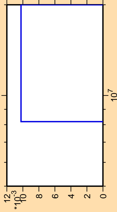
\Delta\sigma/\sigma vs. E for ^{48}\text{Ti}(n,2n\alpha)
