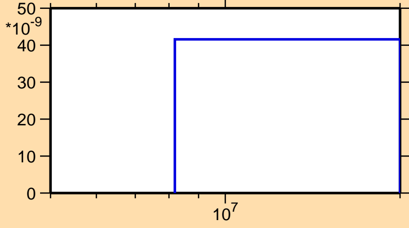
\sigma vs. E for ^{48}\text{Ti}(n,nd)
