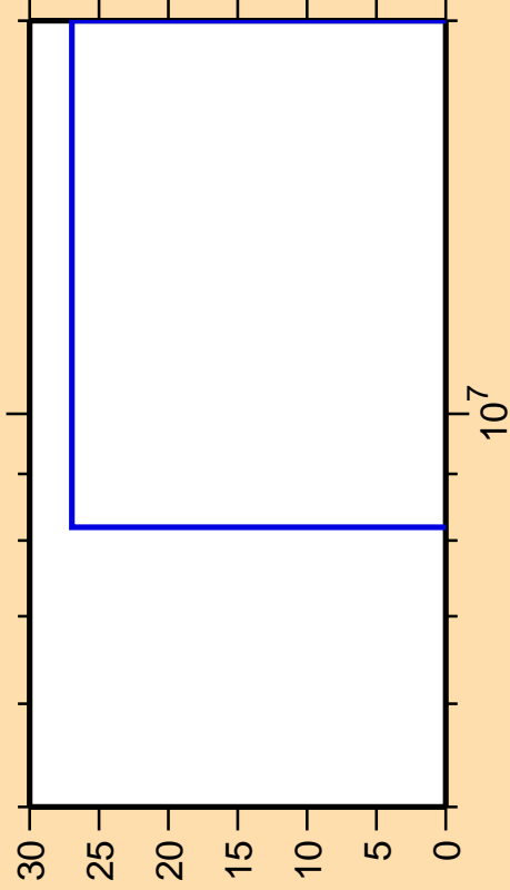
\Delta\sigma/\sigma vs. E for ^{48}\text{Ti}(n,pd)
