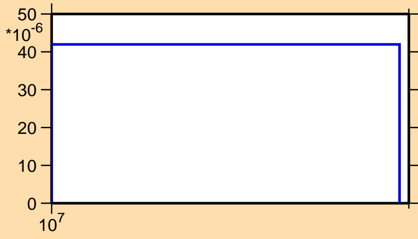
\sigma vs. E for ^{49}\text{Ti}(n,t)
