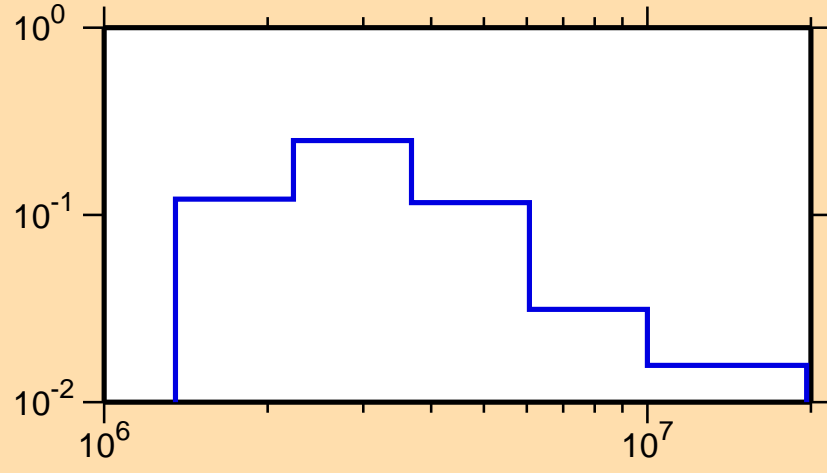
\sigma vs. E for ^{49}\text{Ti}(n,n_4)
