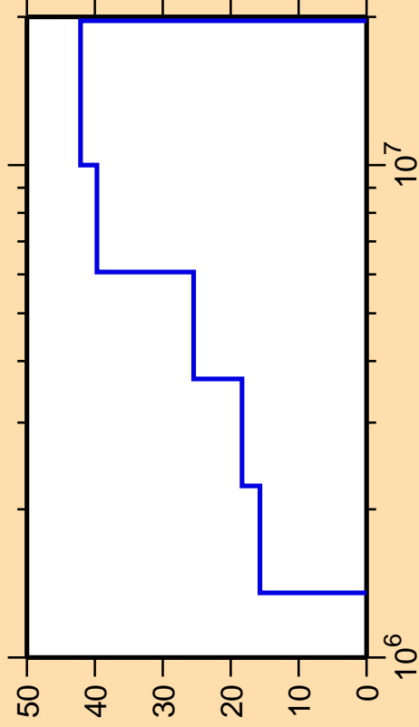
\Delta\sigma/\sigma vs. E for ^{49}\text{Ti}(n,n_2)
