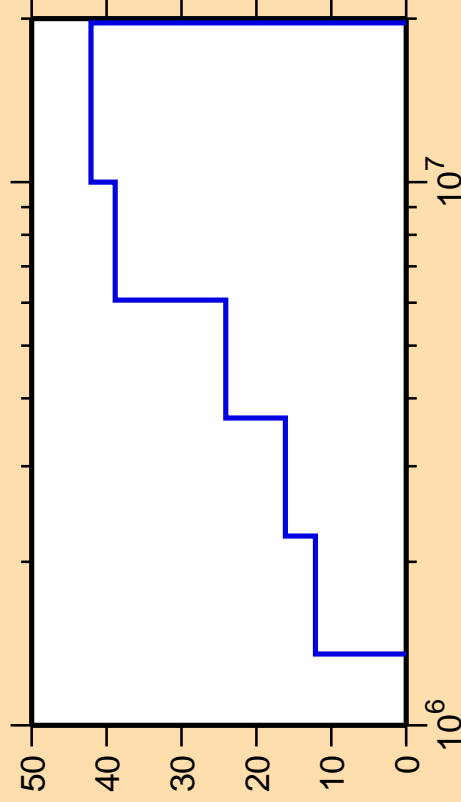
\Delta\sigma/\sigma vs. E for ^{49}\text{Ti}(n,n_4)
