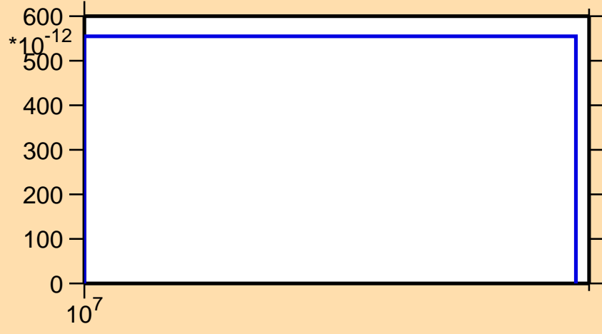
\sigma vs. E for ^{49}\text{Ti}(n,\text{nd})
