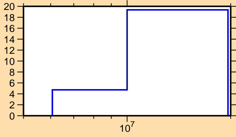
\Delta\sigma/\sigma vs. E for ^{49}\text{Ti}(n,\text{inel.})
