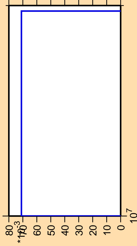
\Delta\sigma/\sigma vs. E for ^{49}\text{Ti}(n,p\alpha)
