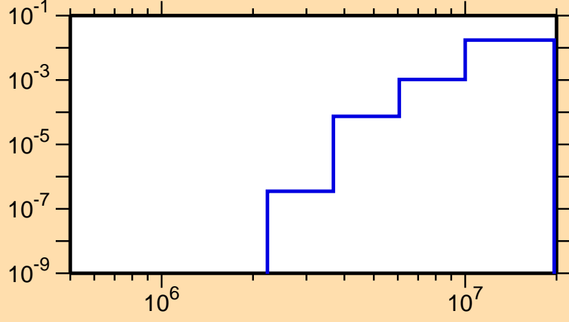
\sigma vs. E for ^{49}\text{Ti}(n,\alpha)
