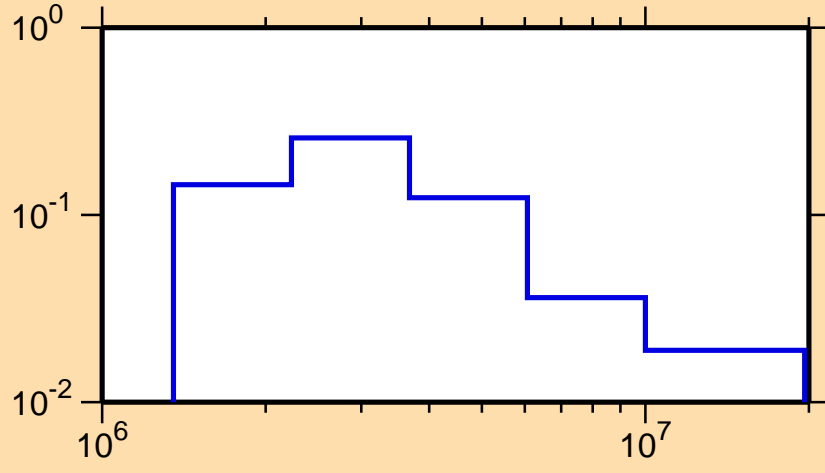
\sigma vs. E for ^{49}\text{Ti}(n,n_2)
