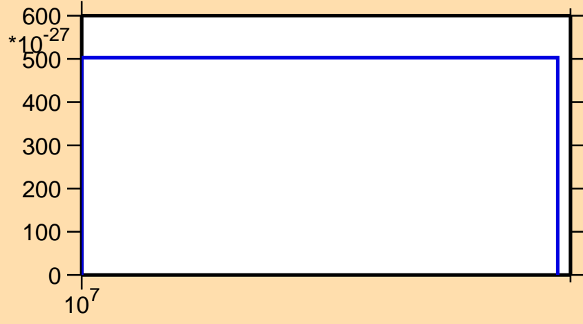
\sigma vs. E for ^{49}\text{Ti}(n,\text{pd})
