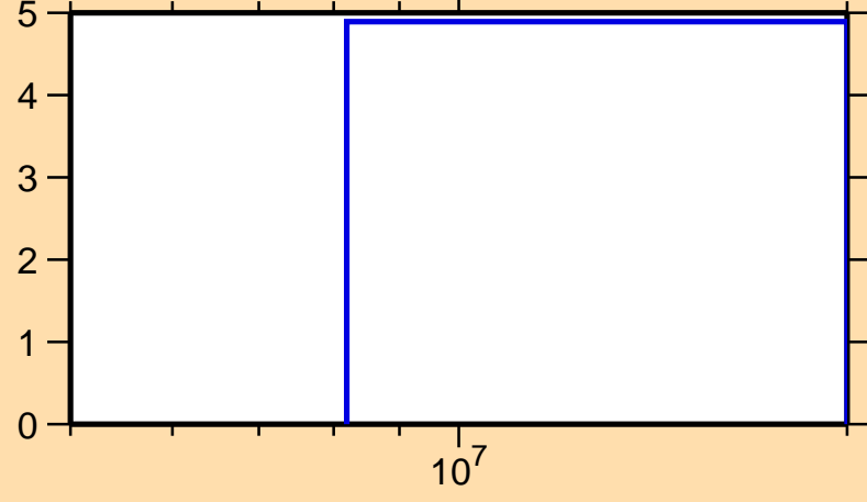
\Delta\sigma/\sigma vs. E for ^{49}\text{Ti}(n,\text{nonel.})
