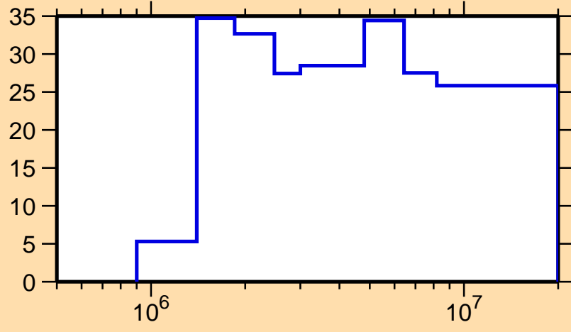
\Delta\sigma/\sigma vs. E for ^{49}\text{Ti}(n,p)
