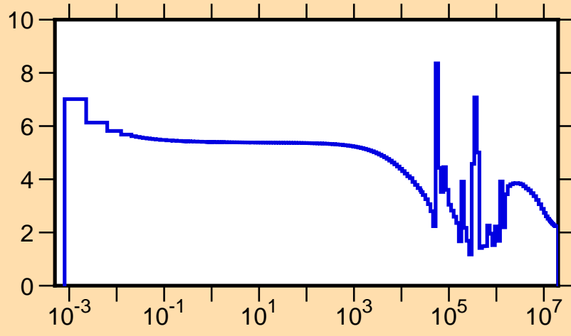
\sigma vs. E for ^{50}\text{Ti}(n,\text{tot.})
