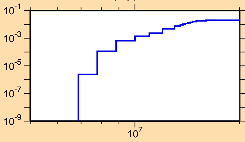
\sigma vs. E for ^{50}\text{Ti}(n,p)
