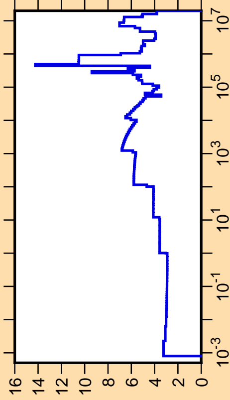
\Delta\sigma/\sigma vs. E for ^{50}\text{Ti}(n,\text{tot.})
