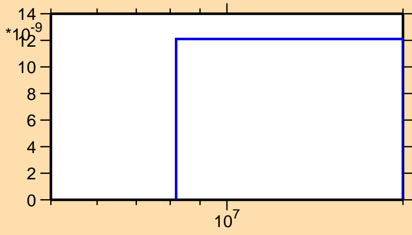
\sigma vs. E for ^{50}\text{Ti}(n,3n)
