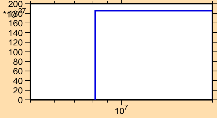
\sigma vs. E for ^{50}\text{Ti}(n,pd)
