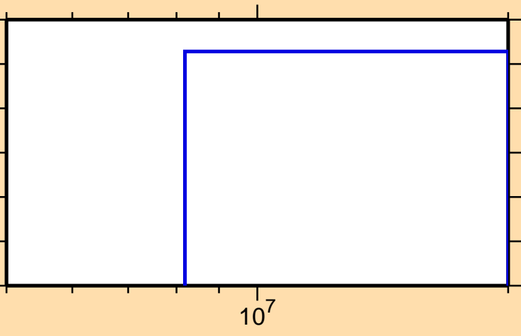
\sigma vs. E for ^{50}\text{Ti}(n,\text{He3})
