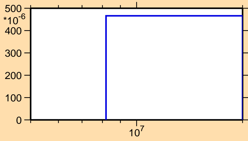
\sigma vs. E for ^{50}\text{Ti}(n,d)
