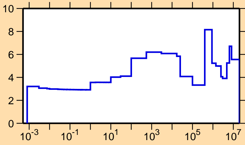
\Delta\sigma/\sigma vs. E for ^{50}\text{Ti}(n,\text{tot.})
