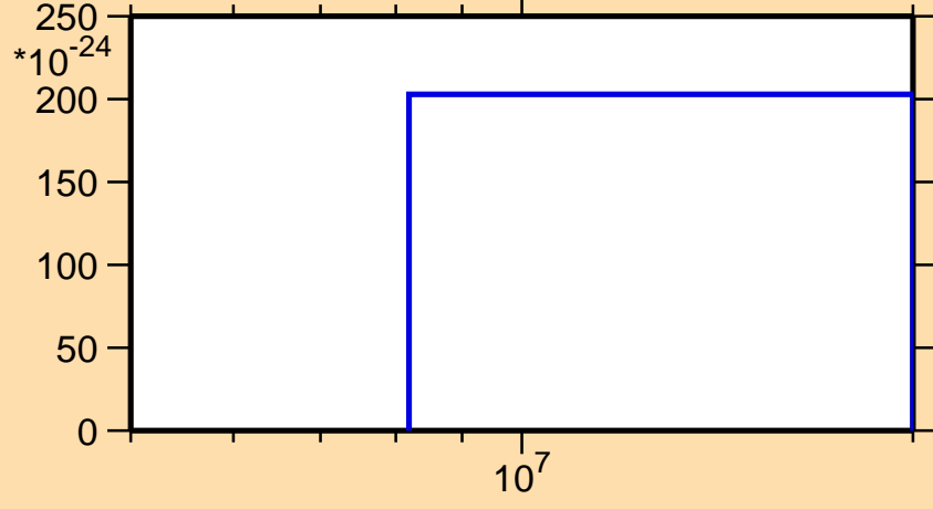
\sigma vs. E for ^{50}\text{Ti}(n,p\alpha)
