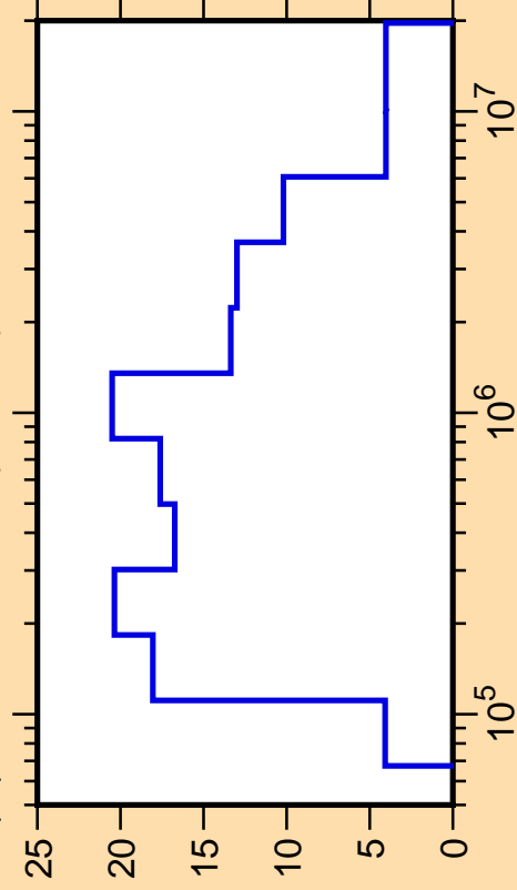
\Delta\mu/\mu vs. E for ^{52}\text{Ti}(\text{mt251})
