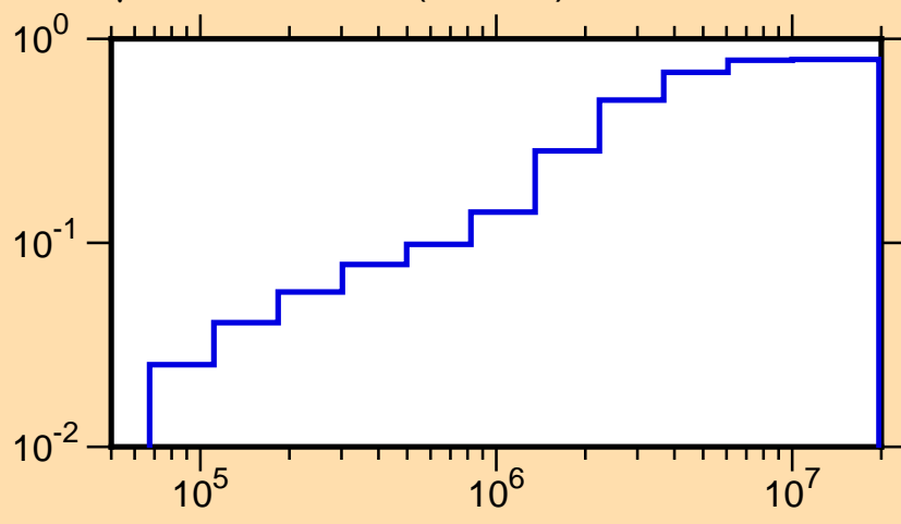
\mu vs. E for ^{52}\text{Ti}(\text{mt251})
