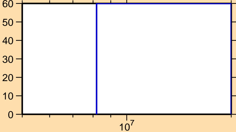
\Delta\sigma/\sigma vs. E for ^{53}\text{Ti}(n,n\text{cont.})
