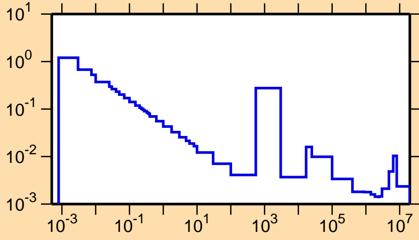
\sigma vs. E for ^{53}\text{Ti}(n,\gamma)
