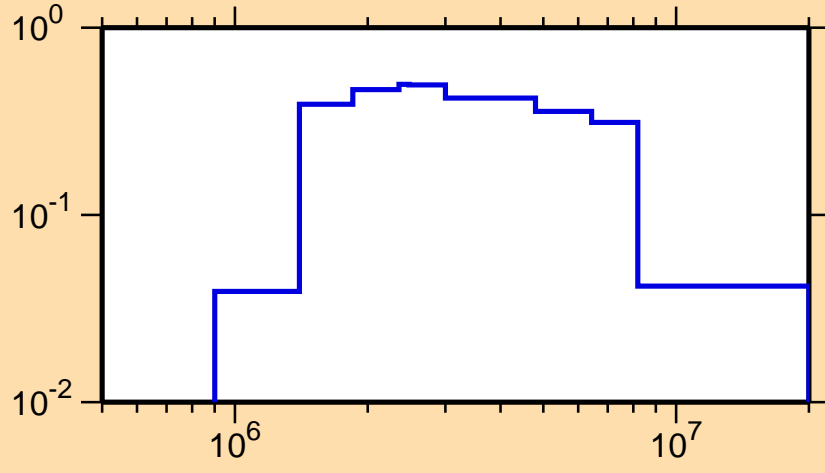
\sigma vs. E for ^{53}\text{Ti}(n,n_1)
