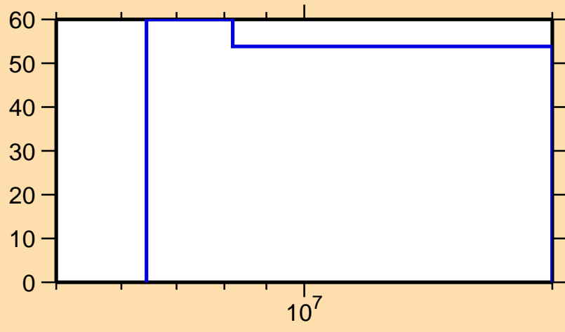
\Delta\sigma/\sigma vs. E for ^{53}\text{Ti}(n,p)
