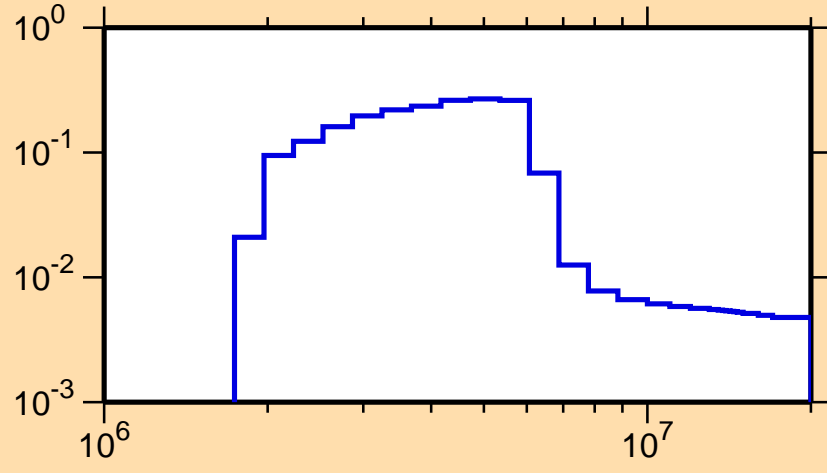
\sigma vs. E for ^{55}\text{Ti}(n,n_3)
