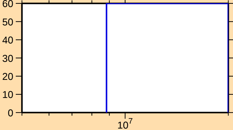
\Delta\sigma/\sigma vs. E for ^{180}\text{Tl}(n,2n)
