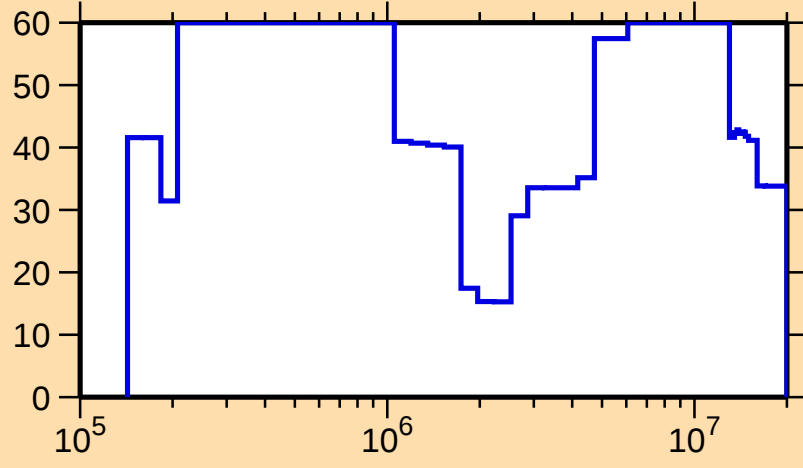
\Delta\sigma/\sigma vs. E for ^{180}\text{Tl}(n,\text{el.})
