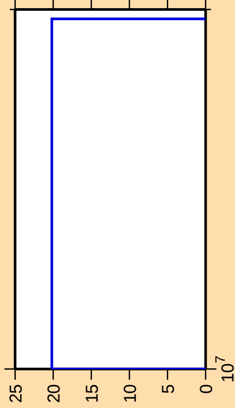
\Delta\sigma/\sigma vs. E for ^{180}\text{Tl}(n,nt)
