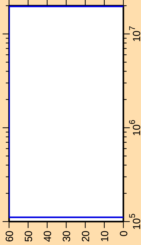
\Delta\sigma/\sigma vs. E for ^{180}\text{Tl}(n,p)
