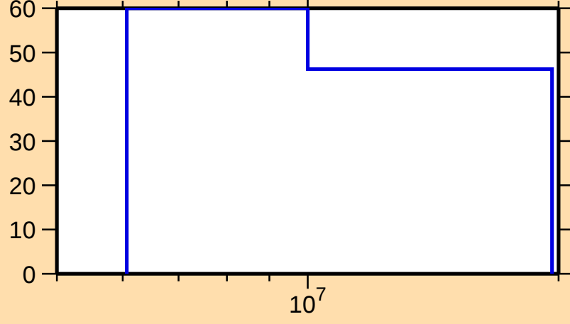
\Delta\sigma/\sigma vs. E for ^{180}\text{Tl}(n,\text{el.})
