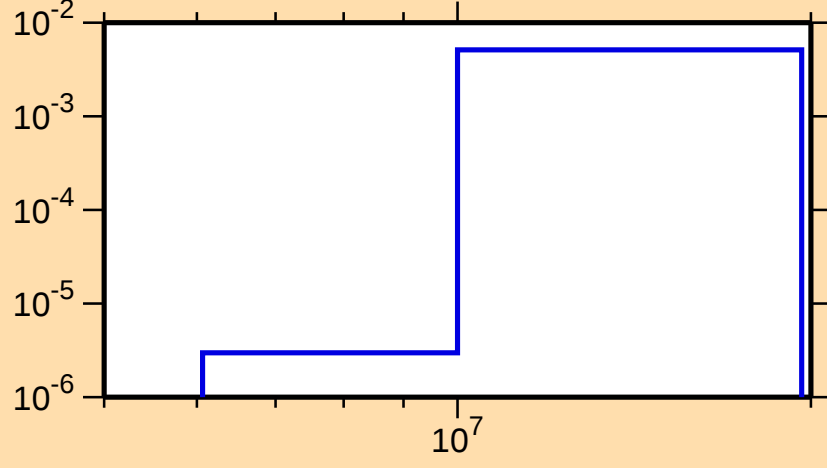
\sigma vs. E for ^{180}\text{Tl}(n,2n\alpha)
