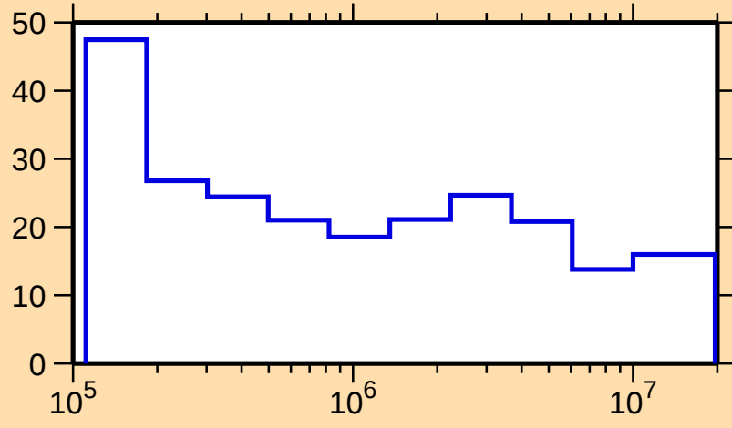
\Delta\sigma/\sigma vs. E for ^{180}\text{Tl}(n,\text{nonel.})
