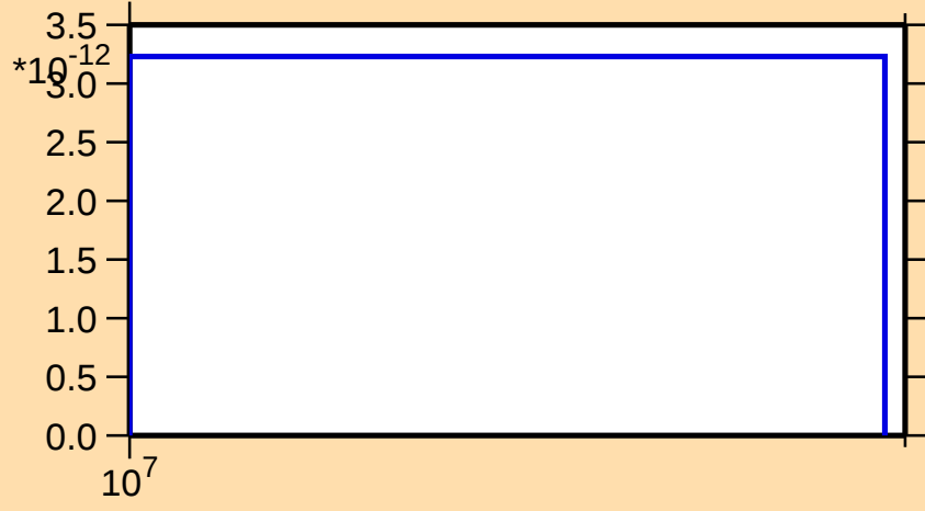
\sigma vs. E for ^{180}\text{Tl}(n,nt)
