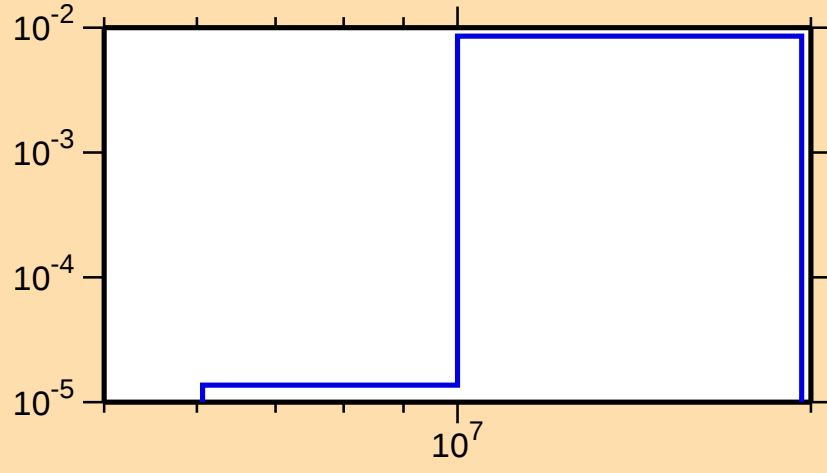
\sigma vs. E for ^{180}\text{Tl}(n,2n)
