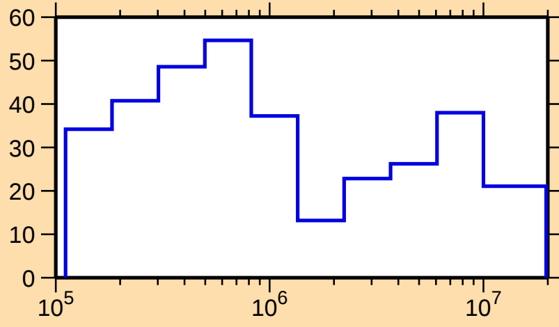
\Delta\sigma/\sigma vs. E for ^{180}\text{Tl}(n,\text{tot.})
