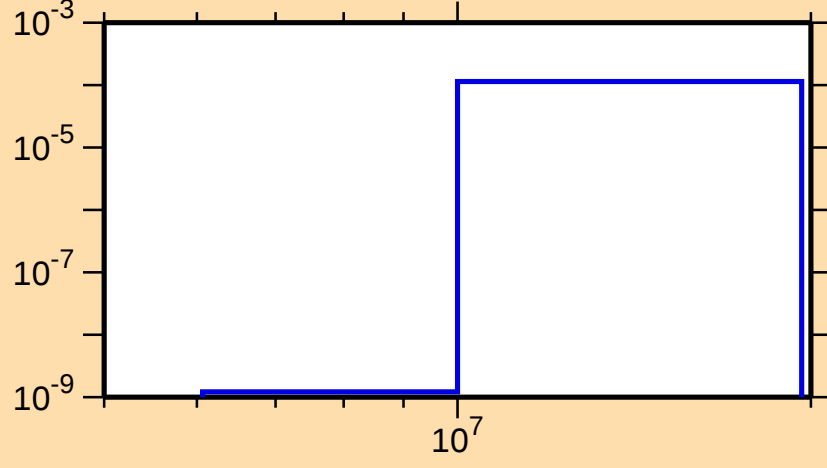
\sigma vs. E for ^{180}\text{Tl}(n,\text{pd})
