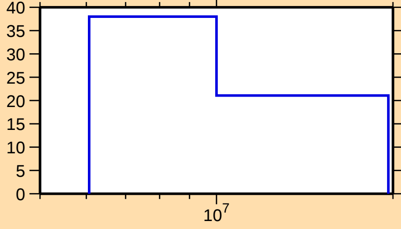
\Delta\sigma/\sigma vs. E for ^{180}\text{Tl}(n,\text{tot.})
