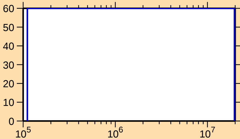
\Delta\sigma/\sigma vs. E for ^{180}\text{Tl}(n,n_1)
