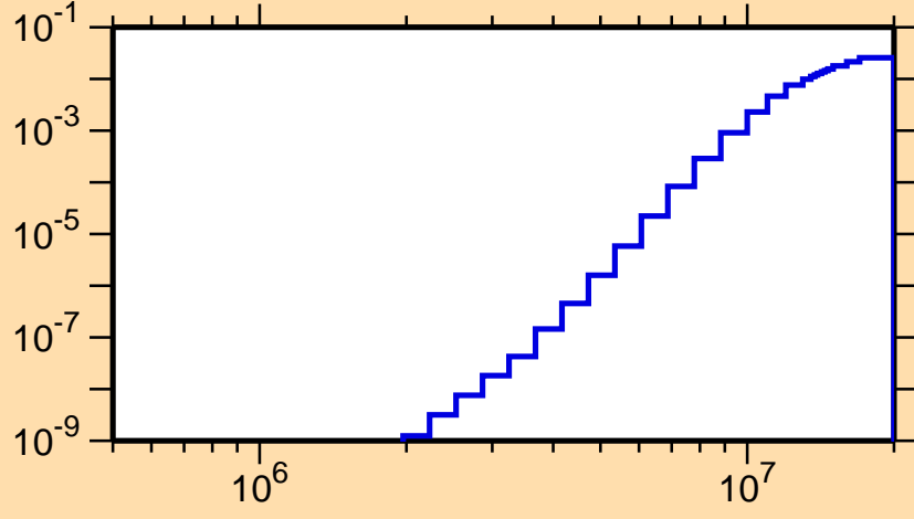
\sigma vs. E for ^{181}\text{Tl}(n,d)
