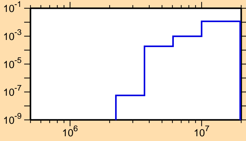
\sigma vs. E for ^{181}\text{Tl}(n,n\alpha)
