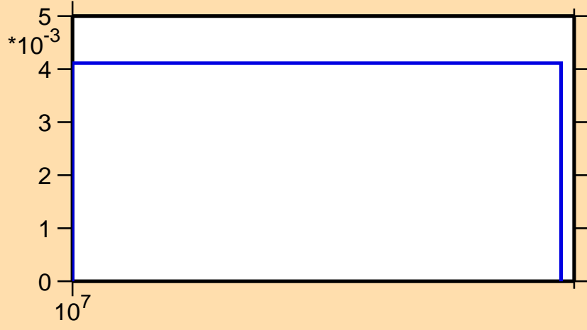
\sigma vs. E for ^{181}\text{Tl}(n,2n)
