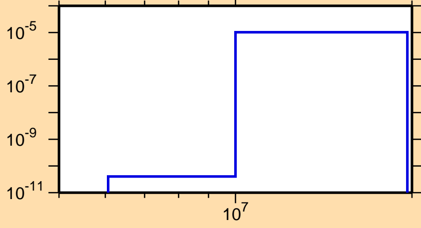
\sigma vs. E for ^{181}\text{Tl}(n,\text{pd})
