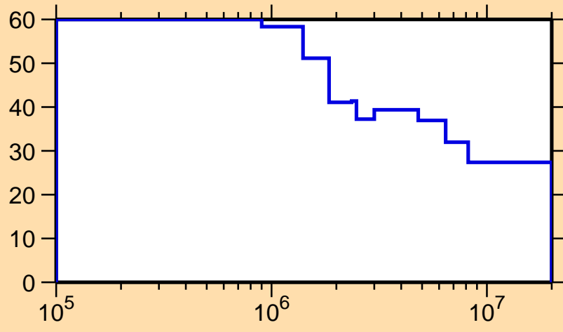
\Delta\sigma/\sigma vs. E for ^{181}\text{Tl}(n,n_1)
