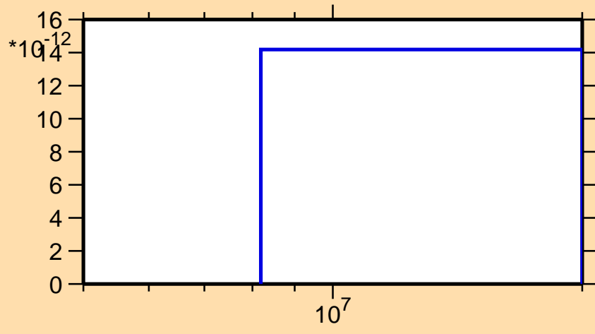
\sigma vs. E for ^{181}\text{Tl} (mt 34)
