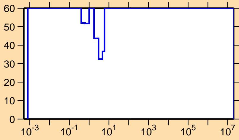
\Delta\sigma/\sigma vs. E for ^{181}\text{Tl}(n,\gamma)
