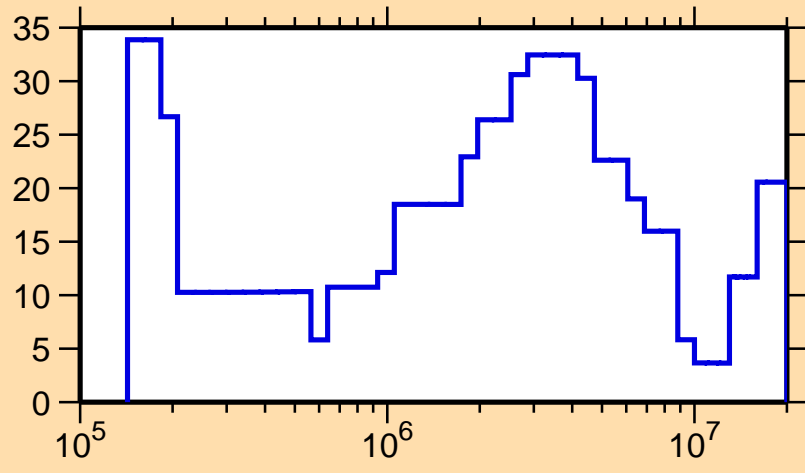
\Delta\sigma/\sigma vs. E for ^{182}\text{Tl}(n, el.)
