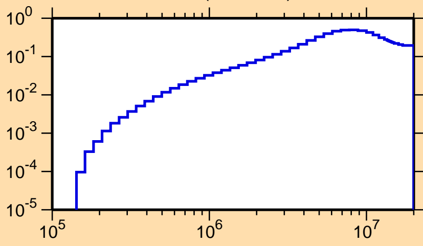
\sigma vs. E for ^{182}\text{Tl}(n,n\text{cont.})
