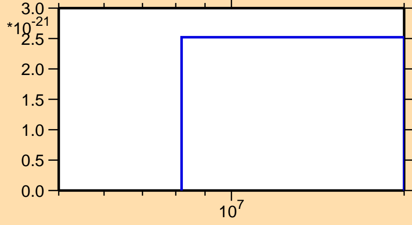
\sigma vs. E for ^{182}\text{Tl} (mt 42)
