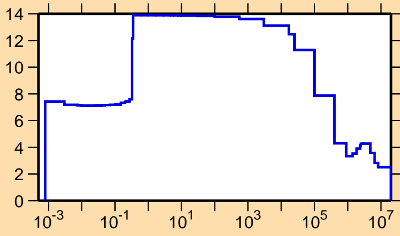
\sigma vs. E for ^{182}\text{Tl}(n,\text{el.})
