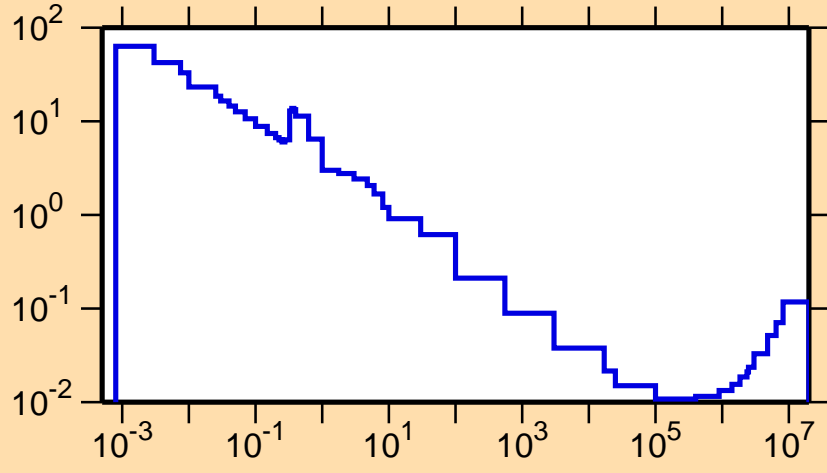
\sigma vs. E for ^{182}\text{Tl}(n,\alpha)
