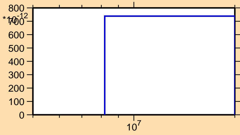
\sigma vs. E for ^{182}\text{Tl}(\text{mt } 34)
