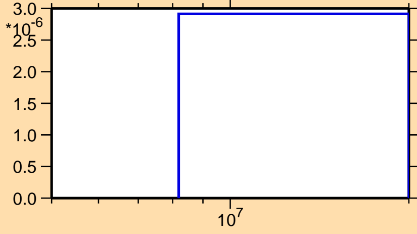
\sigma vs. E for ^{182}\text{Tl}(n,nd)
