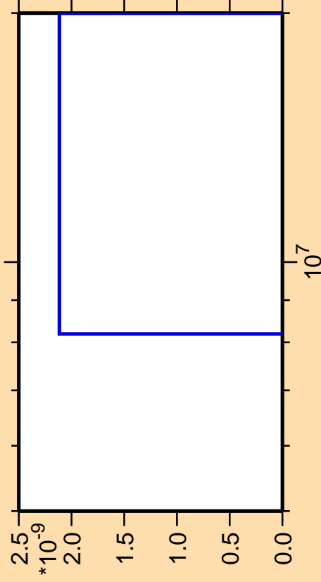
\Delta\sigma/\sigma vs. E for ^{182}\text{Tl} (mt 42)
