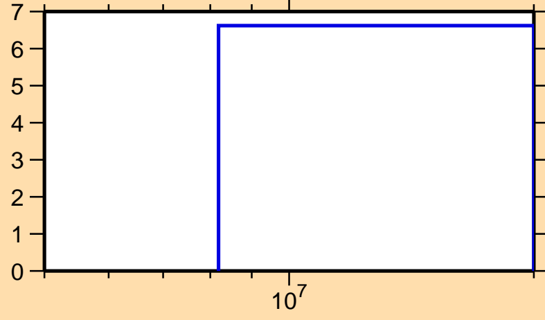
\Delta\sigma/\sigma vs. E for ^{182}\text{Tl}(n,\text{el.})
