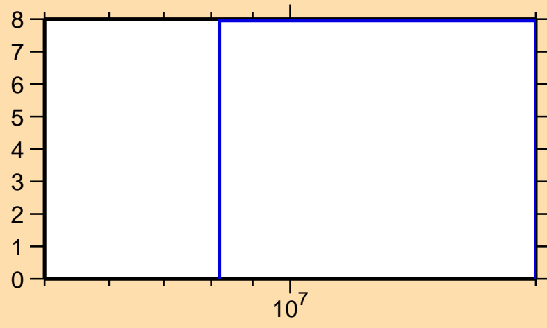
\Delta\sigma/\sigma vs. E for ^{182}\text{Tl}(n,\text{tot.})
