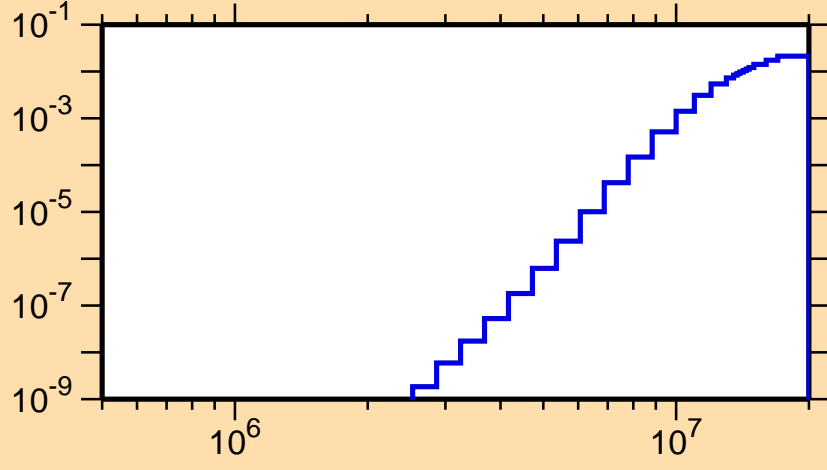
\sigma vs. E for ^{183}\text{Tl}(n,d)
