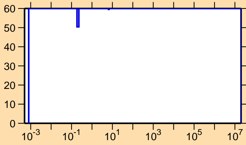
\Delta\sigma/\sigma vs. E for ^{183}\text{Tl}(n,\gamma)
