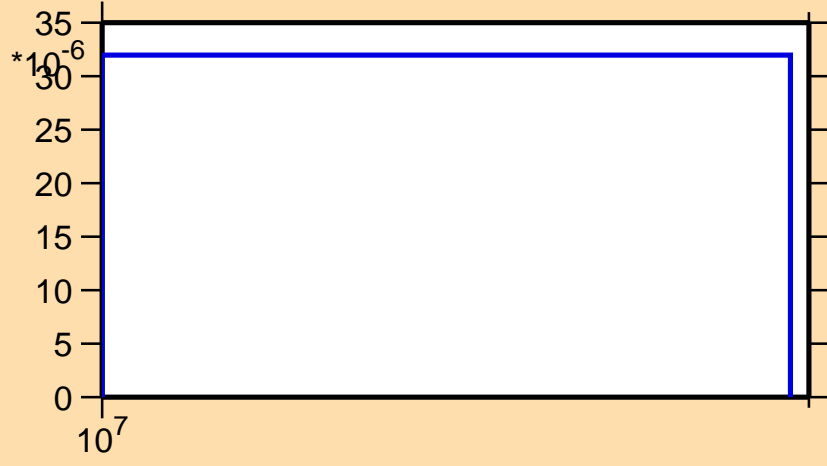
\sigma vs. E for ^{183}\text{Tl}(n,2np)
