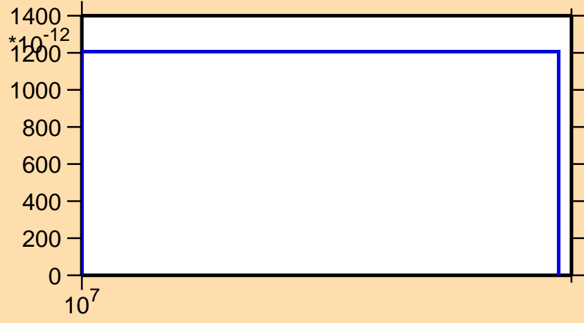
\sigma vs. E for ^{183}\text{Tl}(n,\text{pt})
