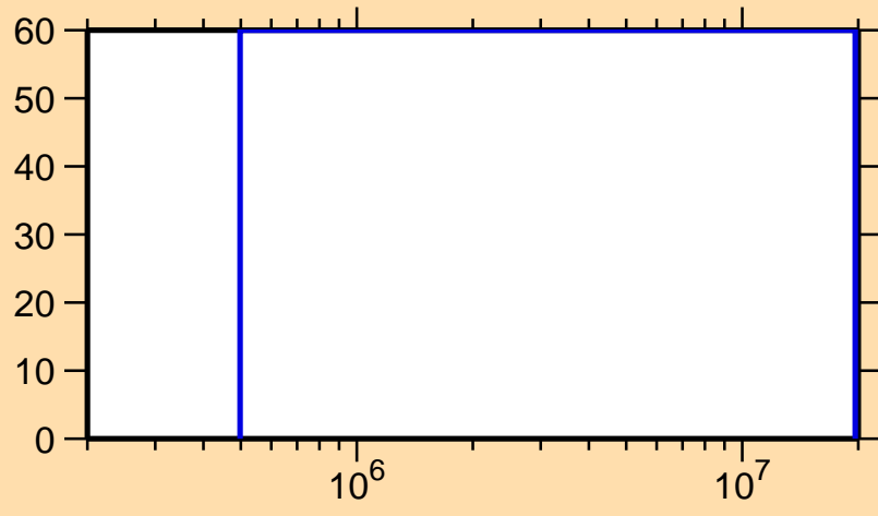
\Delta\sigma/\sigma vs. E for ^{183}\text{Tl}(n,n\text{cont.})
