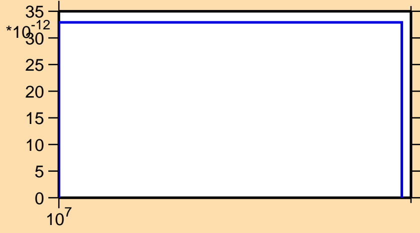
\sigma vs. E for ^{183}\text{Tl}(n,nt)
